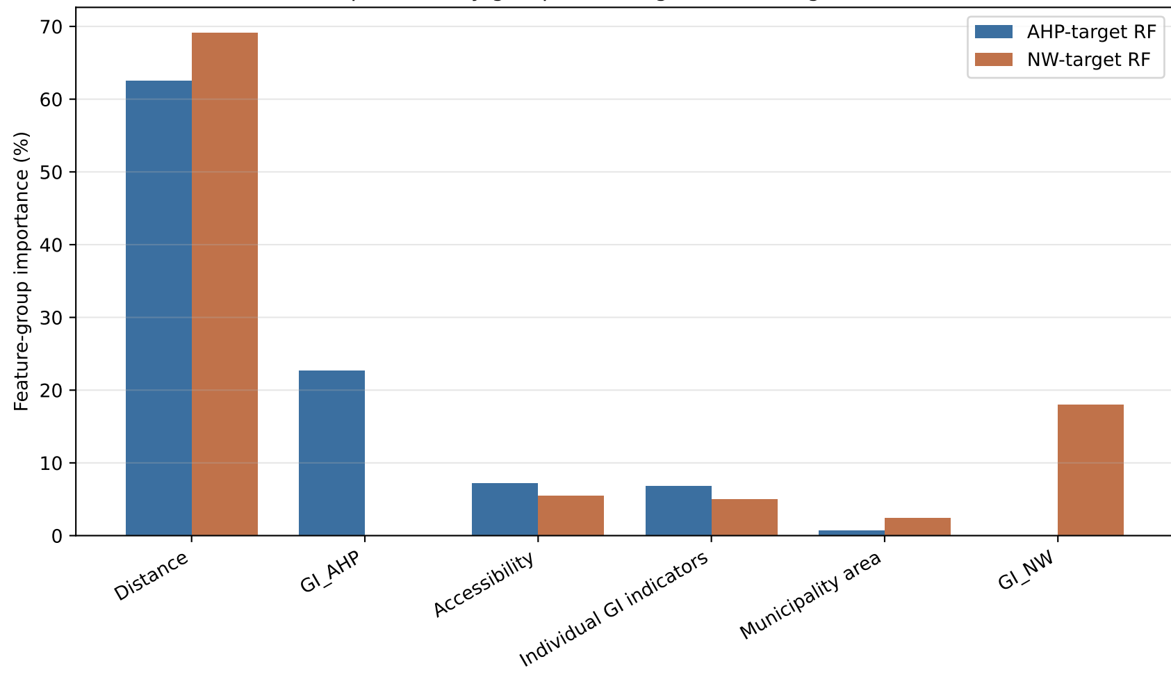
Feature importance by group: AHP-target vs NW-target Random Forest
