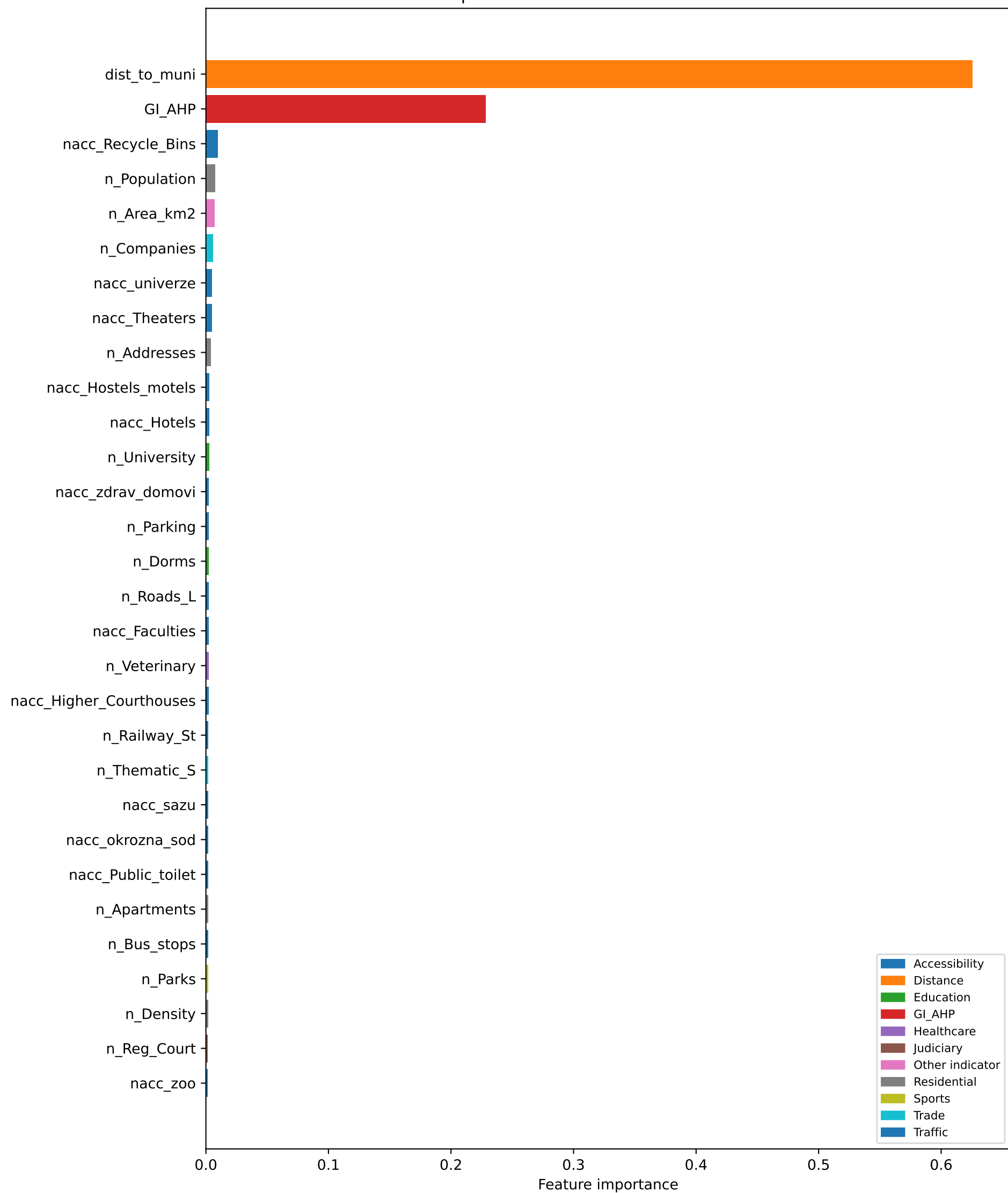
Top 30 features — AHP Random Forest
