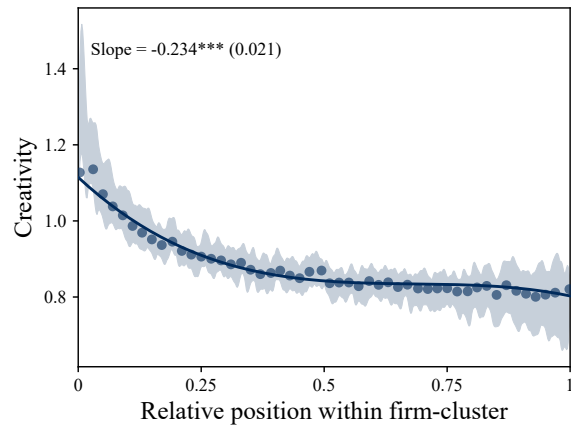
(e) Creativity
