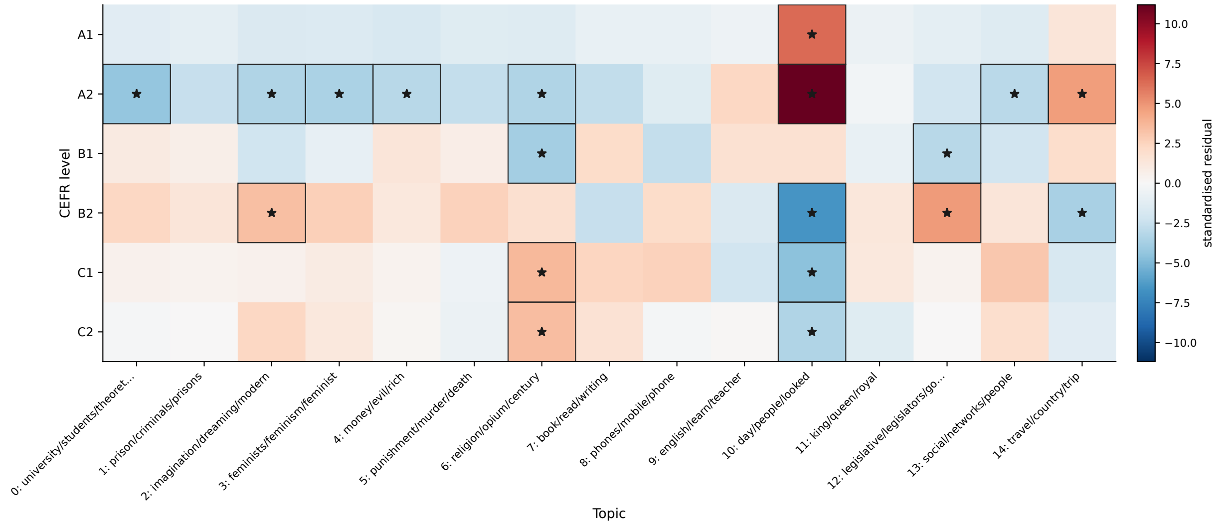
Standardised residuals, topic × level (en)
