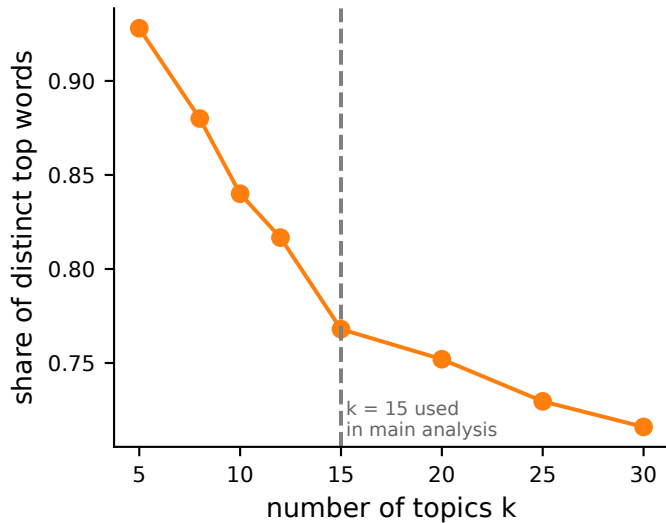
Topic diversity
