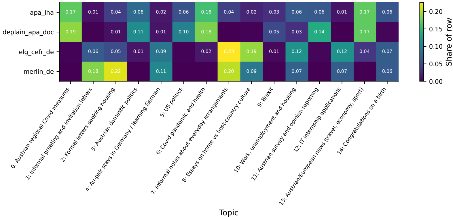
Where each source dataset's texts go, by topic (de)
