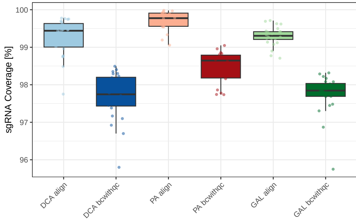
align_UMI_tools vs. bcwithqc – sgRNA Coverage [%]
