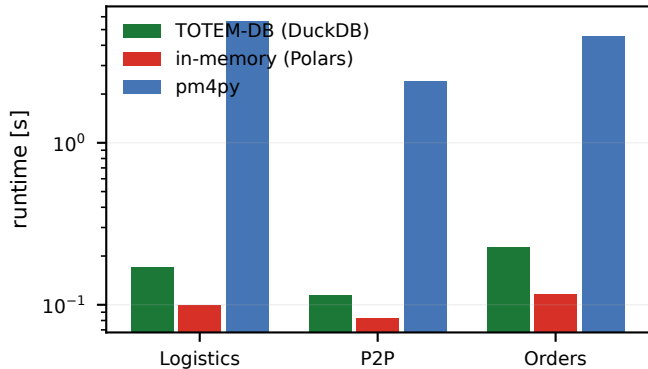
OC-DFG
