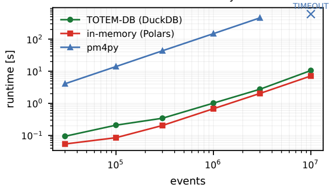
OC-DFG discovery
