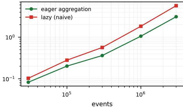
TOTeM: lifetime aggregation
