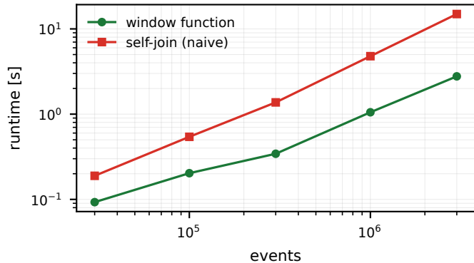
OC-DFG: adjacent-pair formation
