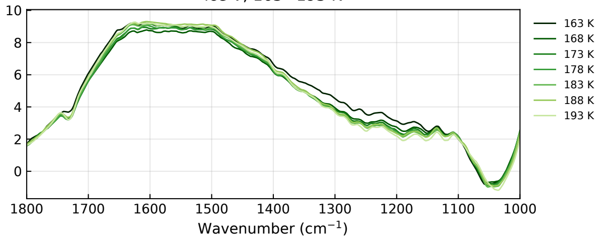
ice V, 163–193 K
