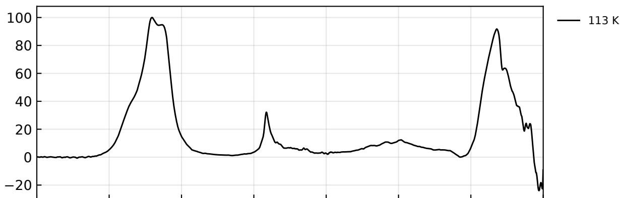
ice I h
