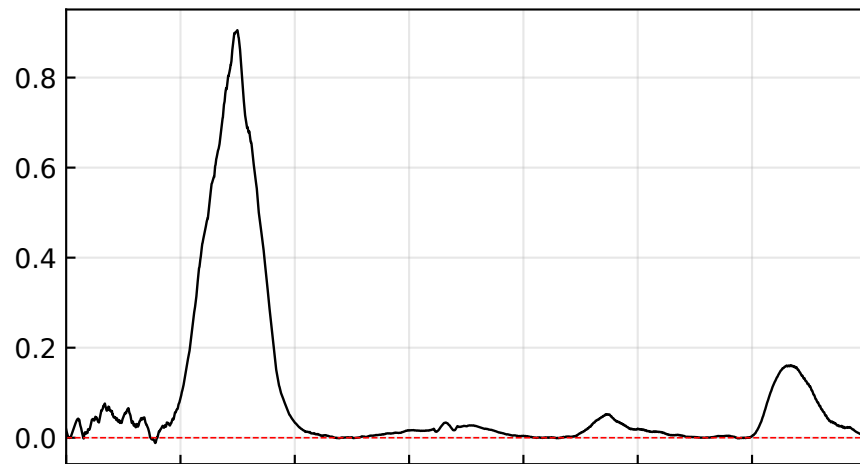
ice Ih: baseline corrected
