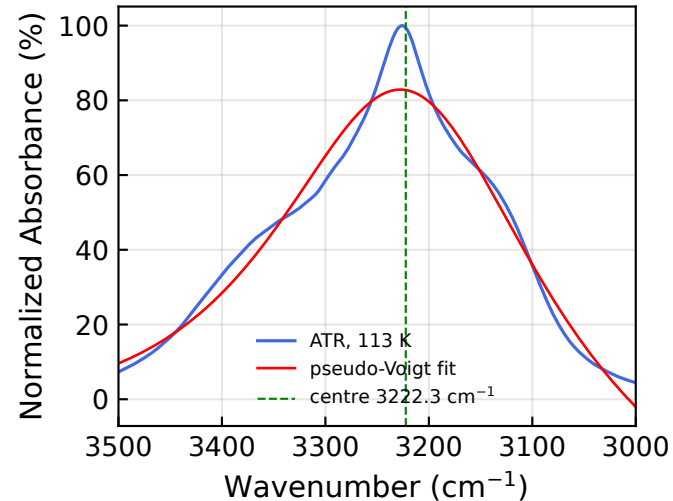
Stretching ( R^2 = 0.965 )
