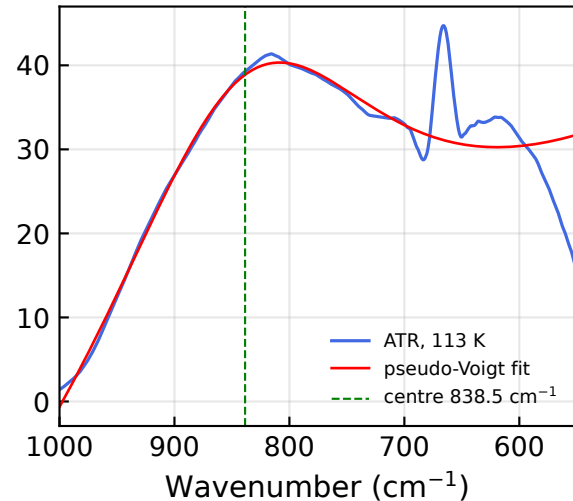
Libration ( R^2 = 0.887 )
