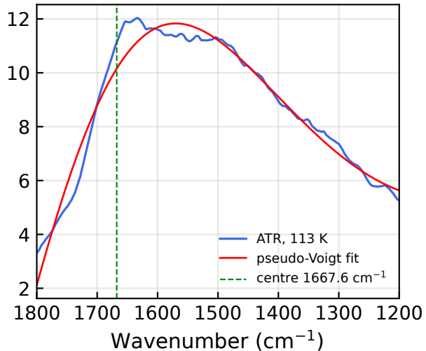
Bending ( R^2 = 0.964 )
