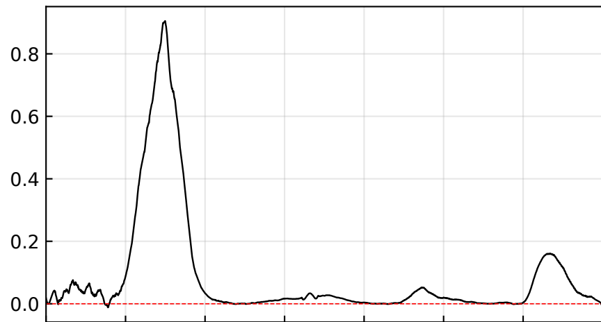
ice Ih: baseline corrected
