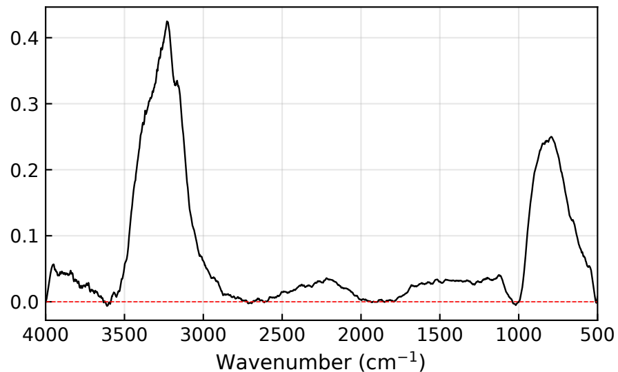
ice Ih: baseline corrected
