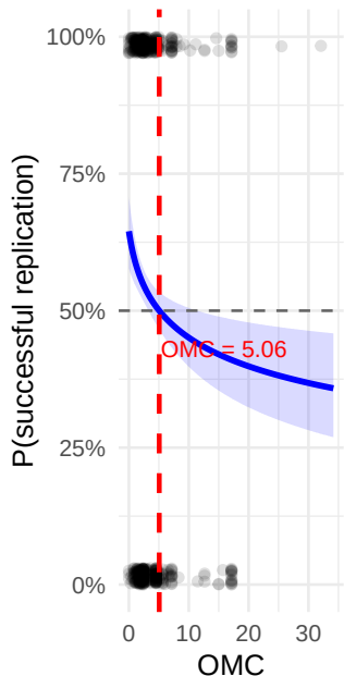
Logistic Regression
