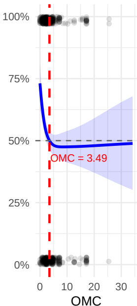
GAM
