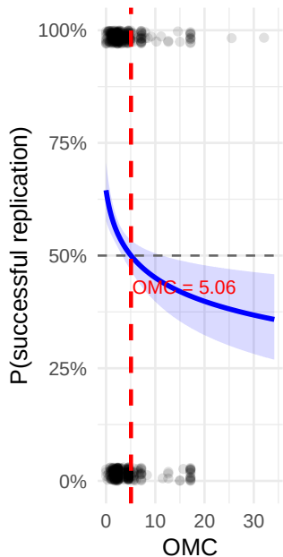
Logistic Regression
