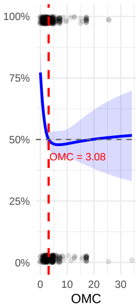
Restricted Cubic Splines
