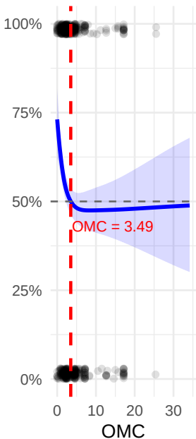
GAM
