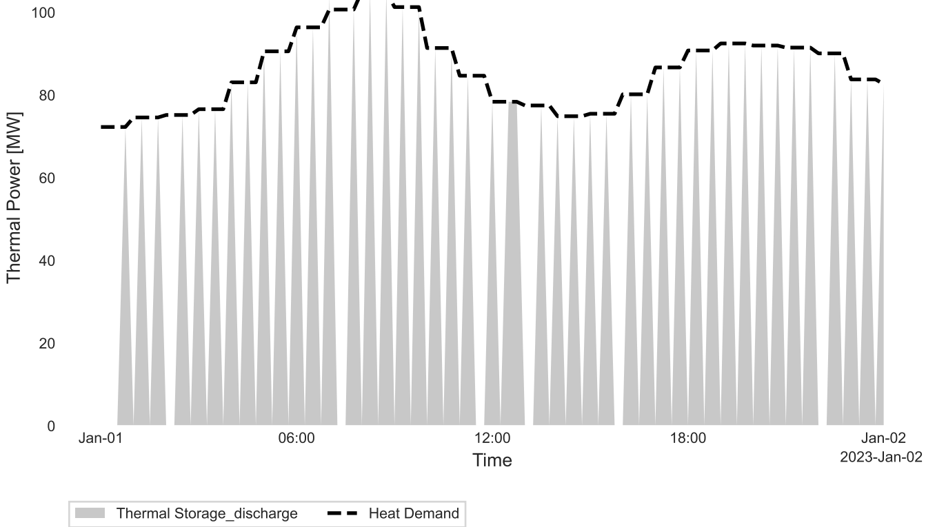
Heat Supply and Demand Balance
