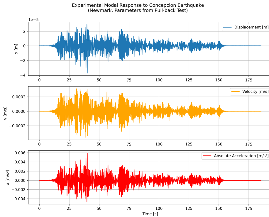
Figure 6: Numerical response of the structure during the Concepción earthquake.
