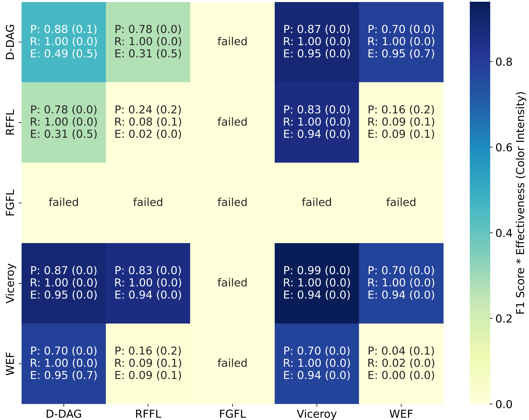
attack=AdvFR, dataset=cifar10, n=100, perc=70%
