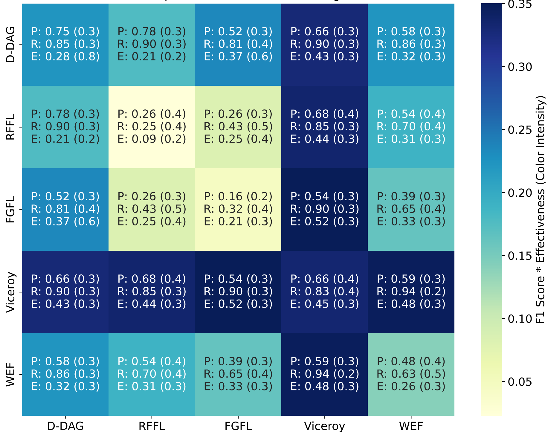
Mean performance accross all settings
