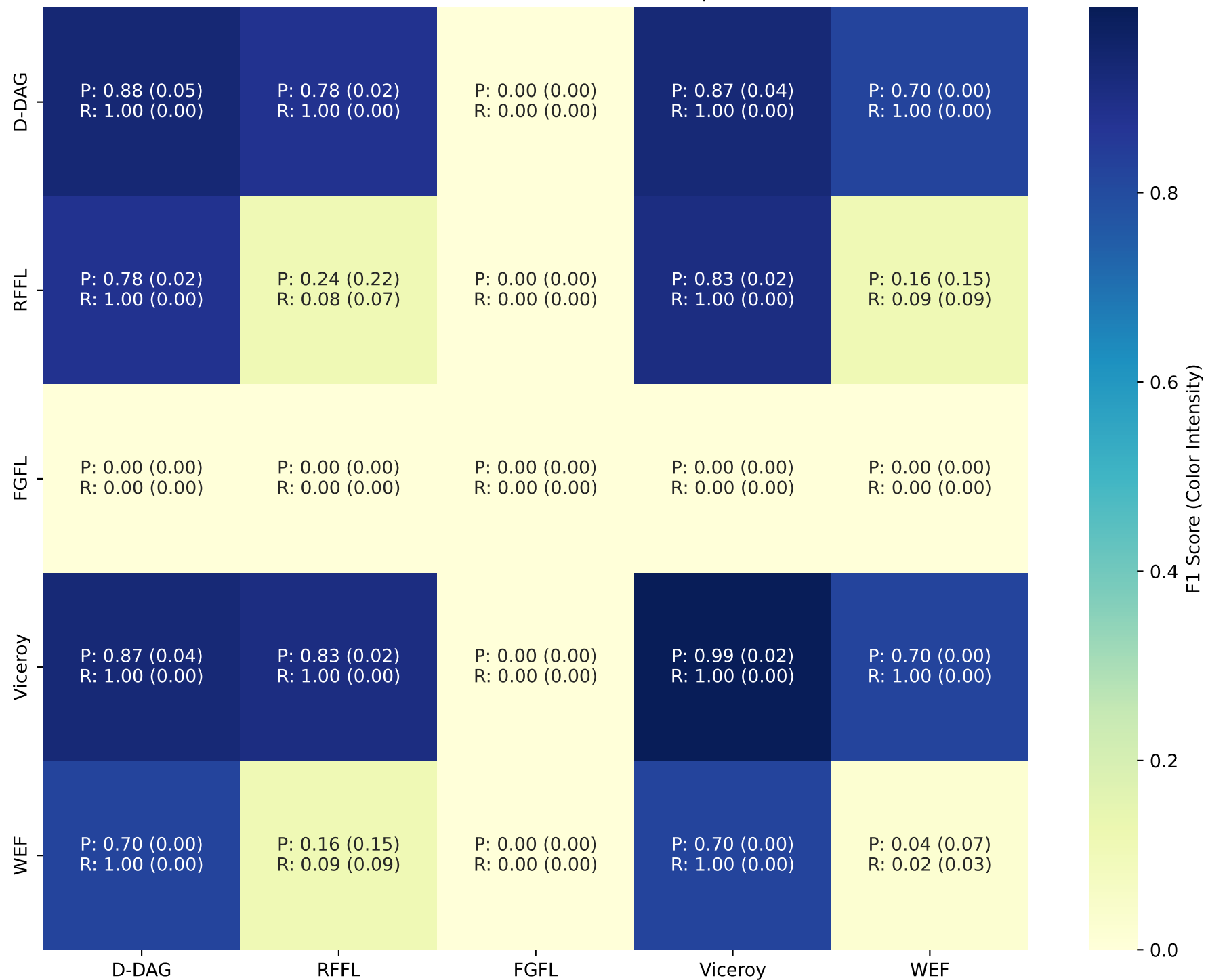
attack=AdvFR, dataset=cifar10, n=100, perc=70%
