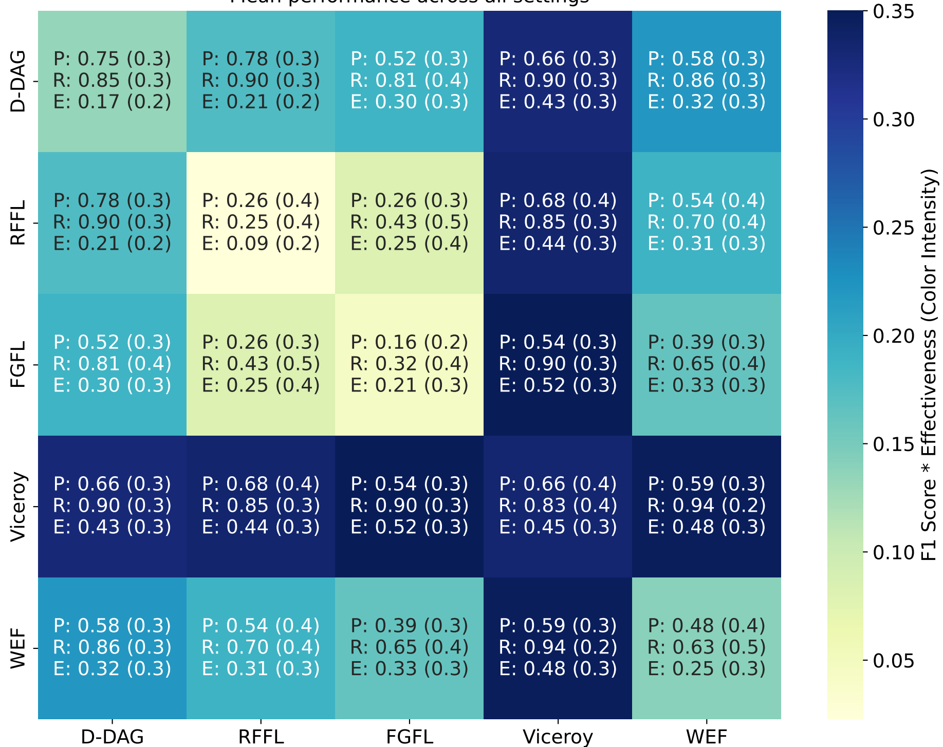
Mean performance across all settings
