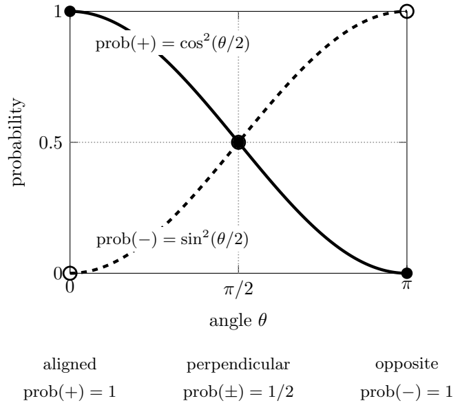
Figure 3: Spin prepared along \mathbf{u}' and measured along \mathbf{u} . Only the angle \theta between the axes enters the probabilities. The solid curve gives the +1/2 outcome; the dashed curve gives the -1/2 outcome. Aligned axes give certainty, perpendicular axes give equal probabilities, and opposite axes reverse the certain outcome. The two curves sum to one at every angle.
