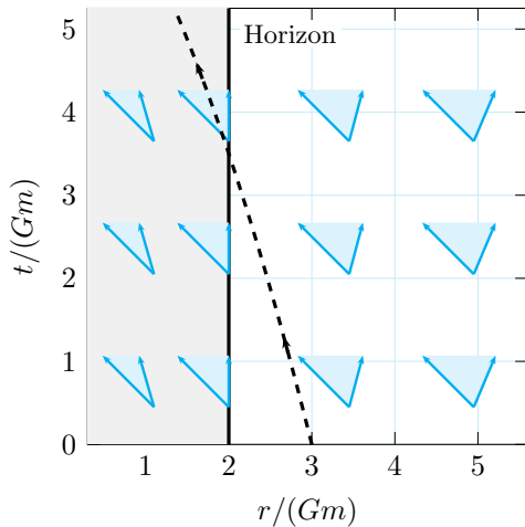
Radial light cones
