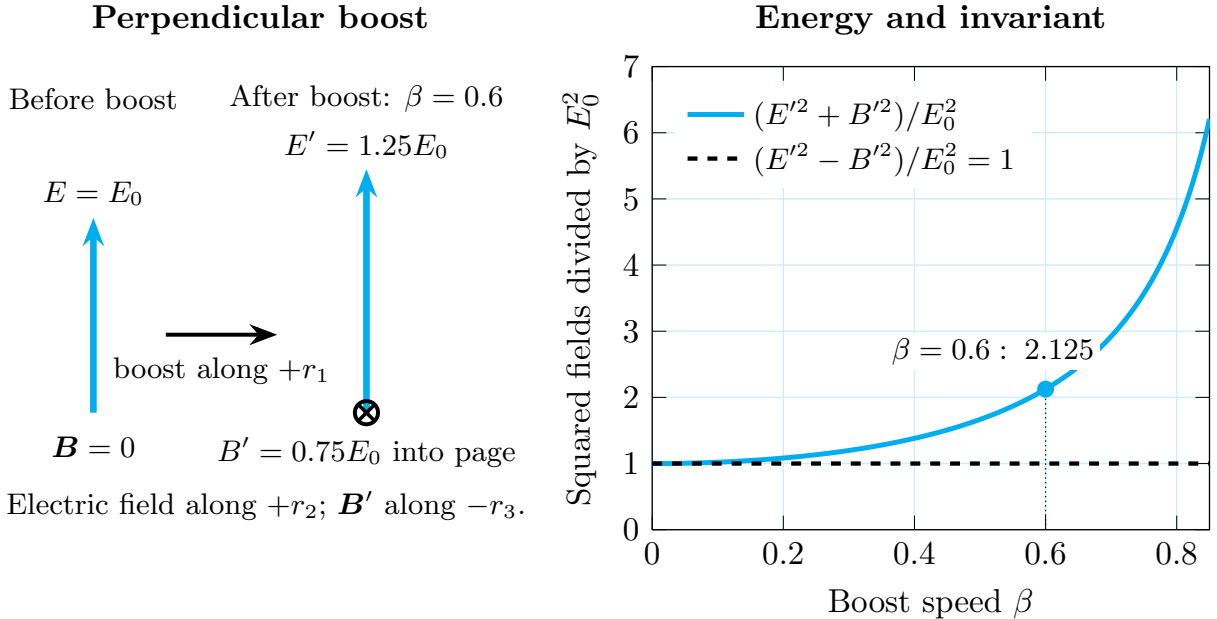
Figure 5: A perpendicular boost of a purely electric field with initial magnitude E_0 \in \mathbb{R}_{>0} . Left: electric arrows are drawn to a common scale for \beta = 0.6 ; the crossed circle denotes the induced magnetic field into the page. Right: writing E' = \|\mathbf{E}'\| and B' = \|\mathbf{B}'\| , both in \mathbb{R}_{\geq 0} , the cyan curve is the energy-density ratio (E'^2 + B'^2)/E_0^2 , whereas the black difference (E'^2 - B'^2)/E_0^2 remains one. The other invariant, \mathbf{E}' \cdot \mathbf{B}' , remains zero.
