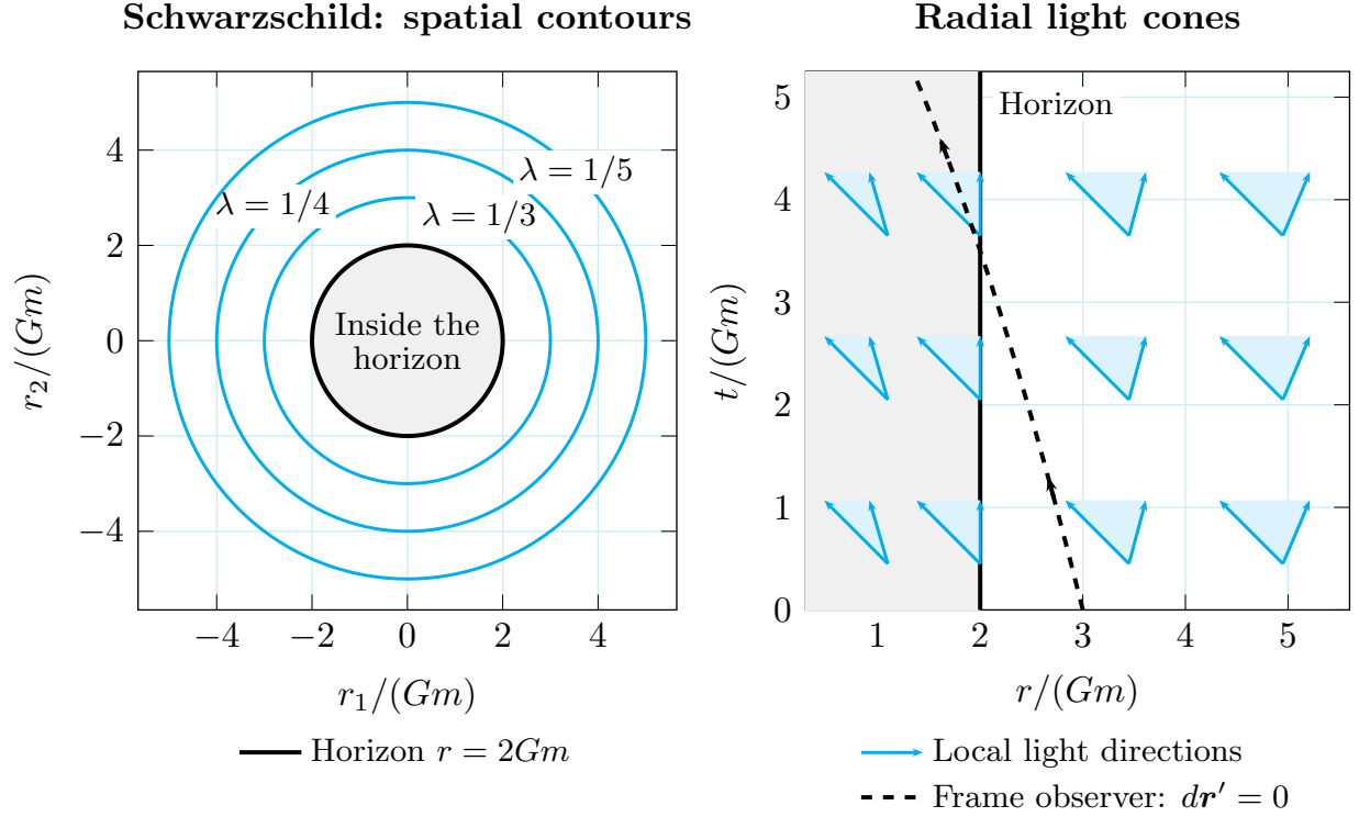
Figure 8: Schwarzschild in the coordinates of (19.28), with lengths and times in units of Gm . Left: constant- \lambda circles in the r_3 = 0 plane; the solid black circle is the horizon, with its interior shaded pale gray. Right: future radial light cones, drawn as local tangent directions, with time increasing upward. The dashed black curve follows the chosen frame observer, dr/dt = -Gm/(r + Gm) , starting at r = 3Gm when t = 0 ; it is not a free-fall trajectory. The spatial panel shows coordinate contours, not proper distances or an isometric embedding.
