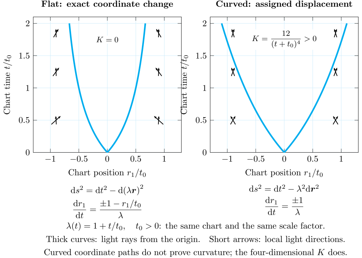
Figure 7: The same positive scale factor \lambda = 1 + t/t_0 , t_0 \in \mathbb{R}_{>0} , used as an exact coordinate rescaling (left) or an assigned local displacement (right). Both diagrams use the same chart, with r_2 = r_3 = 0 . Thick cyan curves are light rays emitted from the origin; short black arrows show local light directions. Curved coordinate paths occur in both panels and do not establish spacetime curvature. Here K \in \mathbb{R}_{\geq 0} is the Kretschmann scalar of the full four-dimensional metric, as in (19.18): only the right metric has nonzero curvature, even though \ddot{\lambda} = 0 .
