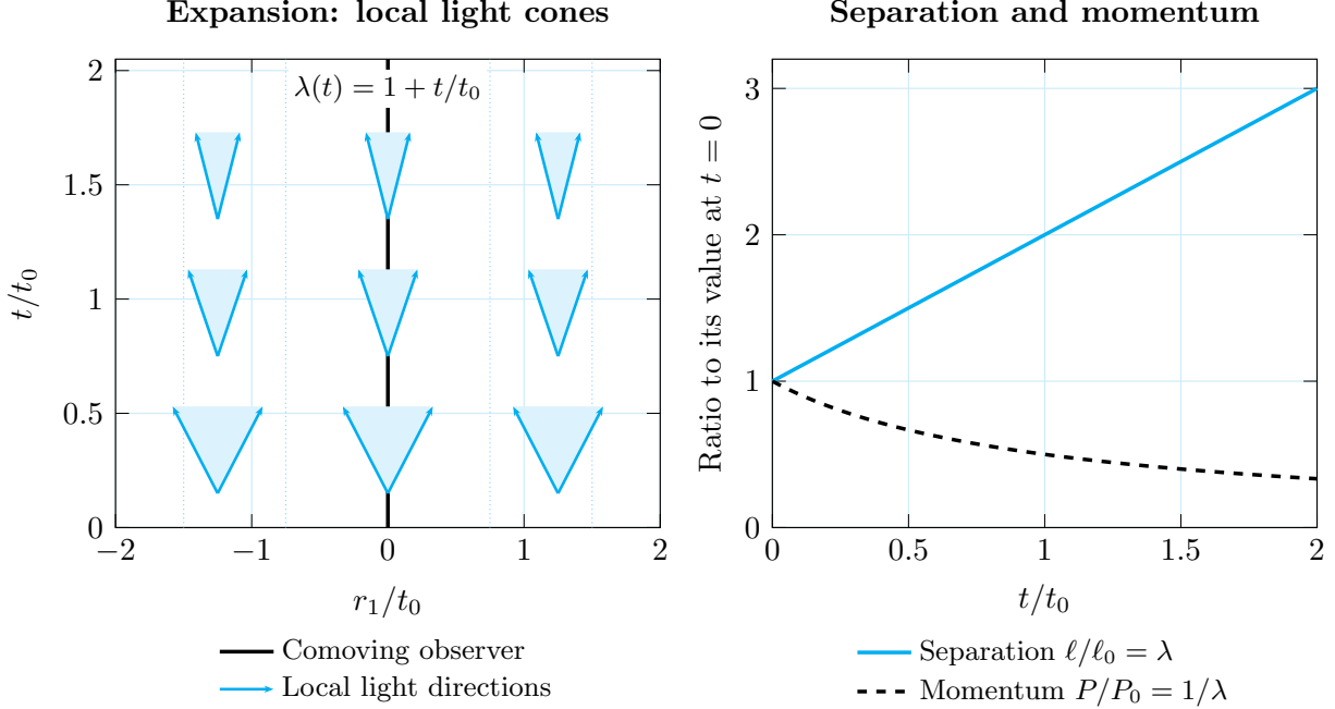
Figure 6: Expansion with \lambda(t) = 1 + t/t_0 , where t_0 \in \mathbb{R}_{>0} . Left: a comoving coordinate slice, with the other spatial coordinates fixed. Cyan arrows are tangent light directions, dr_1/dt = \pm 1/\lambda ; the black line is a comoving observer. Narrowing coordinate cones do not change the locally measured speed of light, which remains one. Right: the physical separation of comoving observers grows as \ell/\ell_0 = \lambda , while a freely moving particle's momentum magnitude P = \|\mathbf{P}\| \in \mathbb{R}_{\geq 0} scales as P/P_0 = 1/\lambda . Subscript zero denotes t = 0 . This illustrative scale factor is not selected by a matter model.
