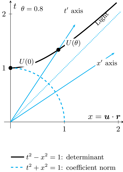
Figure 1: Boost geometry in the t, x plane, with x = \mathbf{u} \cdot \mathbf{r} \in \mathbb{R} . The cyan primed axes have rapidity \theta = 0.8 . The vector U = L^{-2} is the primed frame's unit time direction, expressed in the original coordinates; its components lie on the black unit-determinant hyperbola. The boost takes this vector to rest while preserving the light directions. The cyan unit-norm circle is not preserved. Right: \det U = 1 for every rapidity, whereas \|U\|^2 = \cosh(2\theta) changes.
