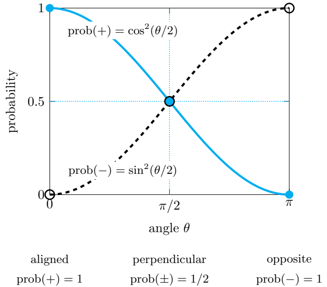
Figure 4: Spin prepared along \mathbf{u}' and measured along \mathbf{u} . Only the angle \theta between the axes enters the probabilities. The cyan solid curve gives the +1/2 outcome; the black dashed curve gives the -1/2 outcome. Aligned axes give certainty, perpendicular axes give equal probabilities, and opposite axes reverse the certain outcome. The two curves sum to one at every angle.
