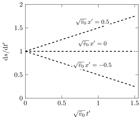
Changing clock-rate differences
