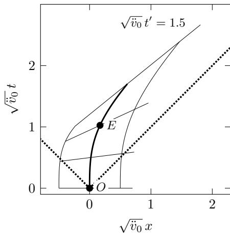
Proper acceleration and jerk
