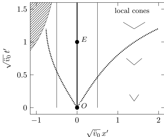
Changing clock-rate differences
