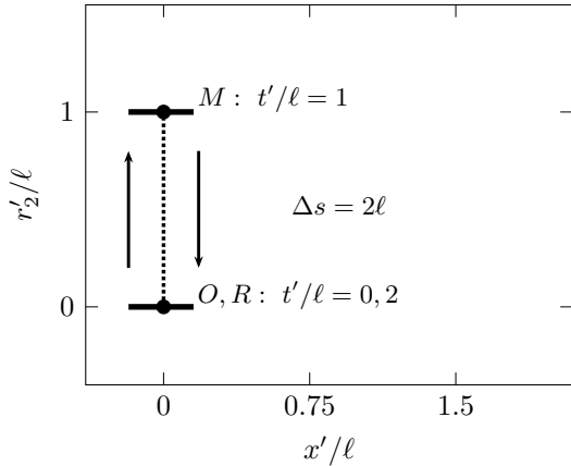
Rest frame: spatial light path
