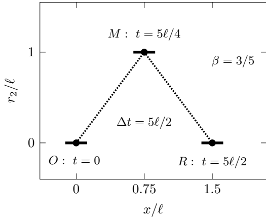
Unprimed frame: moving clock
