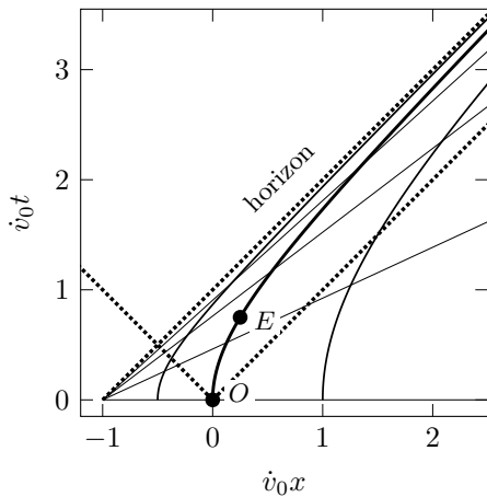
Clocks at fixed grid positions
