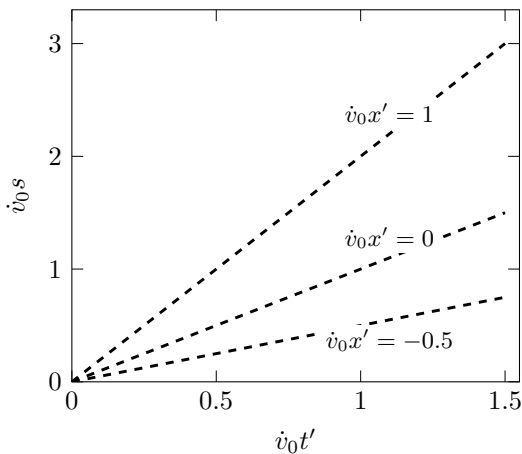
Clocks at fixed grid positions
