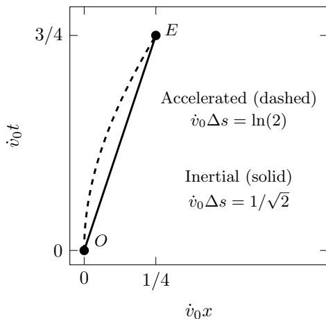
Proper time between O and E
