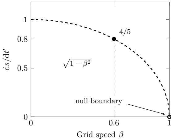
Clock rate on a rotating grid
