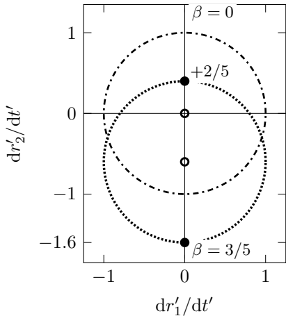
Coordinate light velocities
