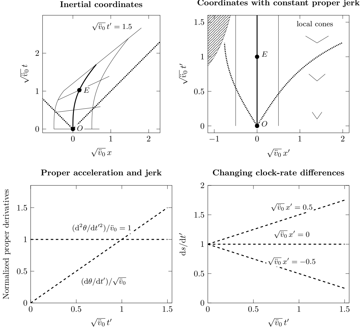
Figure 7: Constant proper jerk from rest and zero initial acceleration, with x = \mathbf{u} \cdot \mathbf{r} and x' = \mathbf{u} \cdot \mathbf{r}' . Top: the same grid and dotted light rays in two coordinate charts. The solid grid worldlines have \sqrt{\ddot{v}_0} x' = -1/2, 0, 1/2 ; thin connecting lines on the left have fixed t' . The shared event E is on the origin at \sqrt{\ddot{v}_0} t' = 1 . The small V shapes on the right show coordinate cones widening with time at a fixed positive x' . Hatching marks failure of 1 + \ddot{v}_0 t' x' > 0 , not by itself a horizon. Bottom: proper acceleration grows linearly, proper jerk stays constant, and the rates of separated grid clocks diverge from their initially common value. All plotted light rays remain null in the inertial chart.
