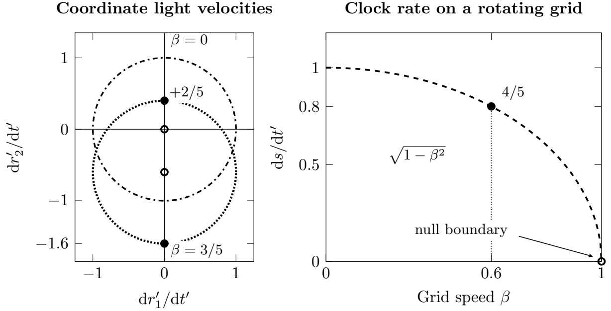
Figure 9: Rotating coordinates with an inertial origin. Left: cross sections of the local coordinate light cone, expressed as velocities in the rotation plane. The dash-dotted circle belongs to the origin ( \beta = 0 ); the dotted circle to a grid point moving with \beta = 3/5 along the second local axis. The tangential coordinate light velocities there are +2/5 and -8/5 ; their different values reflect the rotating axes. Orthonormal measurements still give light speed 1. Right: a clock fixed to that grid point runs at 4/5 of the origin's rate. The open endpoint \beta = 1 marks a null grid worldline, beyond the region occupied by physical rotating-grid clocks.
