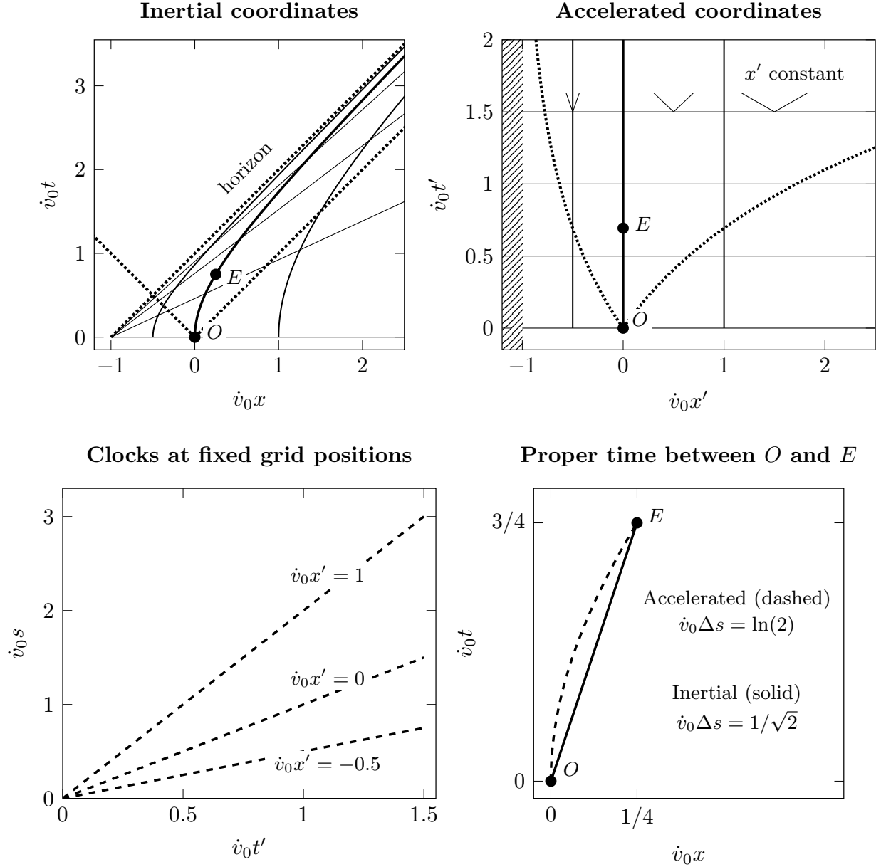
Figure 5: Uniform acceleration, with x = \mathbf{u} \cdot \mathbf{r} and x' = \mathbf{u} \cdot \mathbf{r}' . Top: the same grid and light rays in inertial and accelerated coordinates. The three solid worldlines have \dot{v}_0 x' = -1/2, 0, 1 ; thin connecting lines are simultaneous at fixed t' . Dotted light rays leave O ; the additional dotted null line on the left is the future horizon. Hatching excludes 1 + \dot{v}_0 x' \leq 0 . Short V shapes show local coordinate cones: their width varies with position, while locally measured light speed is 1. Bottom left: fixed grid clocks accumulate different proper times. Bottom right: between the same events O and E : (\dot{v}_0 x, \dot{v}_0 t) = (1/4, 3/4) , the accelerated clock records \ln(2)/\dot{v}_0 , less than the inertial clock's 1/(\sqrt{2}\dot{v}_0) . Thus finite event separation and elapsed time along a curved path differ.
