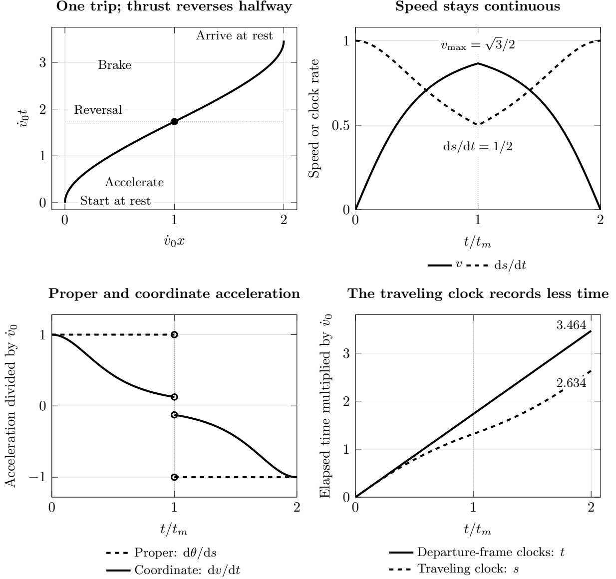
Figure 6: Midpoint braking in flat spacetime, with x = \mathbf{u} \cdot \mathbf{r} \in \mathbb{R} and \dot{v}_0 \ell = 2 . Dotted guides mark the reversal at t = t_m . The trajectory and speed remain continuous while the signed acceleration changes abruptly; open circles show its one-sided values. The proper-acceleration magnitude stays fixed, whereas |\dot{v}| = \dot{v}_0/\gamma^3 varies. The reduced clock rate accumulates to a shorter onboard elapsed time. All plotted axes use the natural units of the main text.
