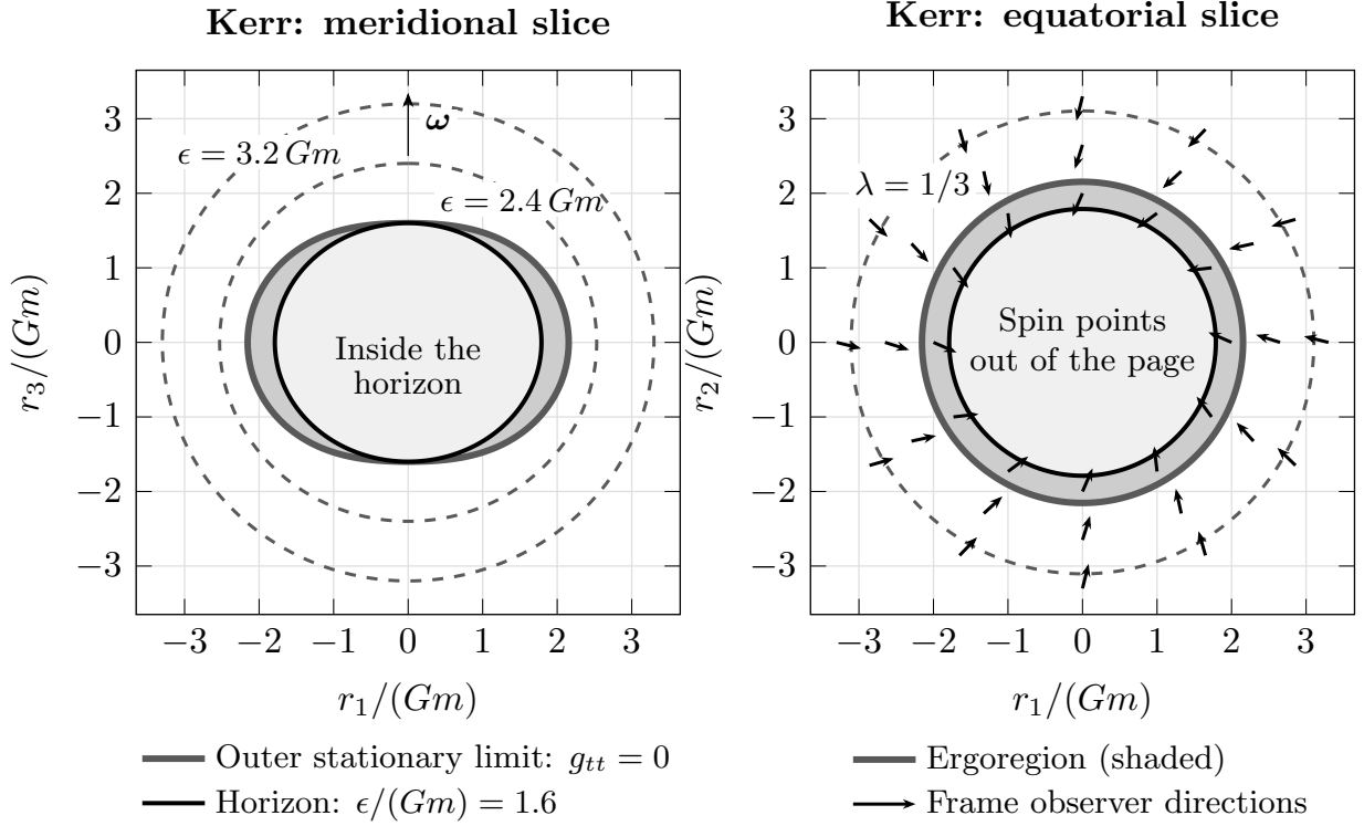
Figure 9: Kerr coordinate slices with spin along +r_3 and Gm\|\omega\| = 1/4 , so \ell^2\|\omega\| = 0.8Gm and the horizon is \epsilon = 1.6Gm . Left: the r_2 = 0 slice, with dashed gray contours of the ellipsoidal radius \epsilon . Right: the r_3 = 0 slice, with a dashed constant- \lambda contour and equal-length arrows showing the direction of d\mathbf{r}/dt = -\lambda\mathbf{u}/(1 + \lambda) . The black outline marks the horizon; the gray outline marks the outer stationary limit. The exterior ergoregion is shaded medium gray; the horizon's interior is light gray. The arrows describe the chosen frame observers, not general free fall; the coordinate shapes are not an isometric embedding.
