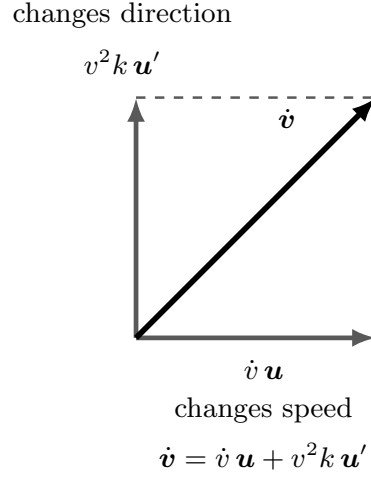
Figure 3: The Frenet frame follows the spatial path. At the marked point, the tangent u and principal normal u' lie in the osculating plane; u'' points out of the page. The dashed osculating circle has radius 1/k . Smaller arrows show how the tangent and normal change along the path. Right: tangential acceleration changes speed, while normal acceleration changes direction. The example is planar, so \tau = 0 ; primes label frame vectors, not derivatives.
