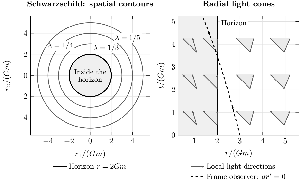
Figure 8: Schwarzschild in the coordinates of (19.28), with lengths and times in units of Gm . Left: constant- \lambda circles in the r_3 = 0 plane; the black circle is the horizon, with its interior shaded light gray. Right: future radial light cones, drawn as local tangent directions, with time increasing upward. The dashed black curve follows the chosen frame observer, dr/dt = -Gm/(r + Gm) , starting at r = 3Gm when t = 0 ; it is not a free-fall trajectory. The spatial panel shows coordinate contours, not proper distances or an isometric embedding.
