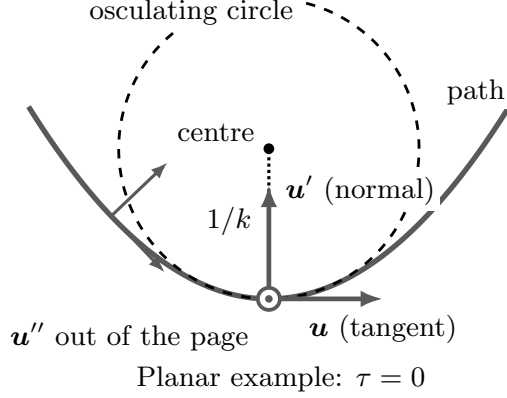
Figure 3: The Frenet frame follows the spatial path. At the marked point, the tangent u and principal normal u' lie in the osculating plane; u'' points out of the page. The dashed osculating circle has radius 1/k . Smaller arrows show how the tangent and normal change along the path. Right: tangential acceleration changes speed, while normal acceleration changes direction. The example is planar, so \tau = 0 ; primes label frame vectors, not derivatives.
