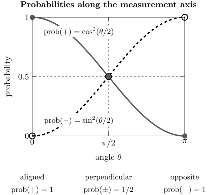
Figure 4: Spin prepared along \mathbf{u}' and measured along \mathbf{u} . Only the angle \theta between the axes enters the probabilities. The solid curve gives the +1/2 outcome; the dashed curve gives the -1/2 outcome. Aligned axes give certainty, perpendicular axes give equal probabilities, and opposite axes reverse the certain outcome. The two curves sum to one at every angle.
