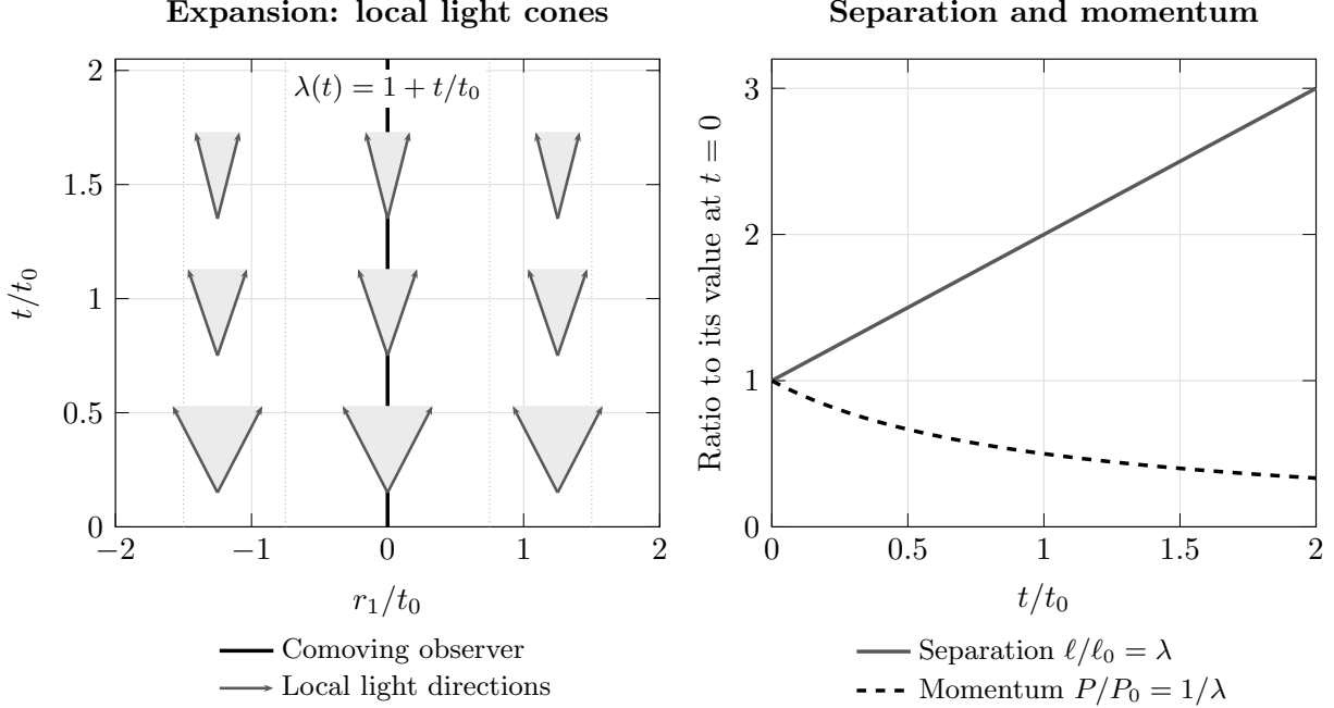
Figure 6: Expansion with \lambda(t) = 1 + t/t_0 , where t_0 > 0 . Left: a comoving coordinate slice, with the other spatial coordinates fixed. Gray arrows are tangent light directions, dr_1/dt = \pm 1/\lambda ; the black line is a comoving observer. Narrowing coordinate cones do not change the locally measured speed of light, which remains one. Right: the physical separation of comoving observers grows as \ell/\ell_0 = \lambda , while a freely moving particle's momentum magnitude P = \|\mathbf{P}\| scales as P/P_0 = 1/\lambda . Subscript zero denotes t = 0 . This illustrative scale factor is not selected by a matter model.
