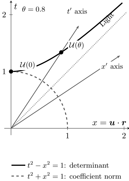
Figure 1: Boost geometry in the t, x plane, with x = \mathbf{u} \cdot \mathbf{r} . The gray primed axes have rapidity \theta = 0.8 . The vector \mathcal{U} = \mathcal{L}^{-2} is the primed frame's unit time direction, expressed in the original coordinates; its components lie on the solid black unit-determinant hyperbola. The boost takes this vector to rest while preserving the light directions. The dashed unit-norm circle is not preserved. Right: \det \mathcal{U} = 1 for every rapidity, whereas \|\mathcal{U}\|^2 = \cosh(2\theta) changes.
