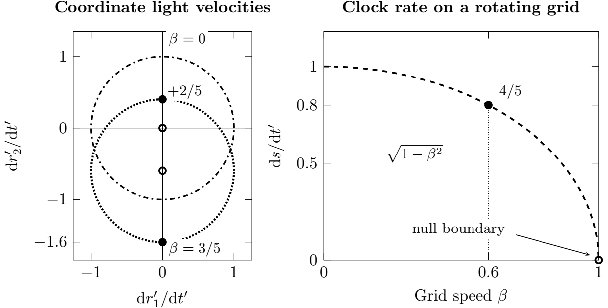
Figure 6: Rotating coordinates with an inertial origin. Left: cross sections of the local coordinate light cone, expressed as velocities in the rotation plane. The dash-dotted circle belongs to the origin ( \beta = 0 ); the dotted circle to a grid point moving with \beta = 3/5 along the second local axis. The tangential coordinate light velocities there are +2/5 and -8/5 ; their different values reflect the rotating axes. Orthonormal measurements still give light speed 1. Right: a clock fixed to that grid point runs at 4/5 of the origin's rate. The open endpoint \beta = 1 marks a null grid worldline, beyond the region occupied by physical rotating-grid clocks.
