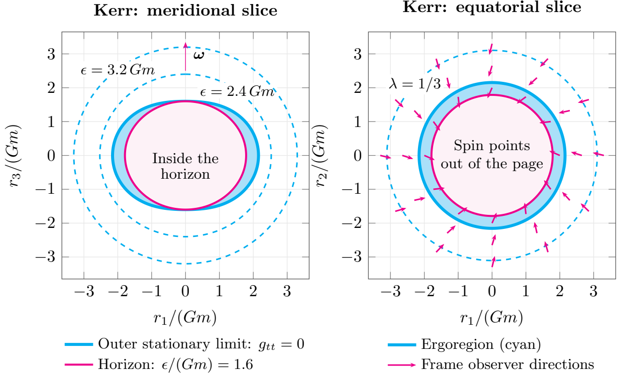
Figure 3: Kerr coordinate slices with spin along +r_3 and Gm\|\omega\| = 1/4 , so \ell^2\|\omega\| = 0.8Gm and the horizon is \epsilon = 1.6Gm . Left: the r_2 = 0 slice, with dashed cyan contours of the ellipsoidal radius \epsilon . Right: the r_3 = 0 slice, with a dashed constant- \lambda contour and equal-length arrows showing the direction of d\mathbf{r}/dt = -\lambda\mathbf{u}/(1 + \lambda) . Solid magenta marks the horizon; solid cyan marks the outer stationary limit, with the exterior ergoregion shaded pale cyan. Pale magenta marks the horizon's interior. The arrows describe the chosen frame observers, not general free fall; the coordinate shapes are not an isometric embedding.
