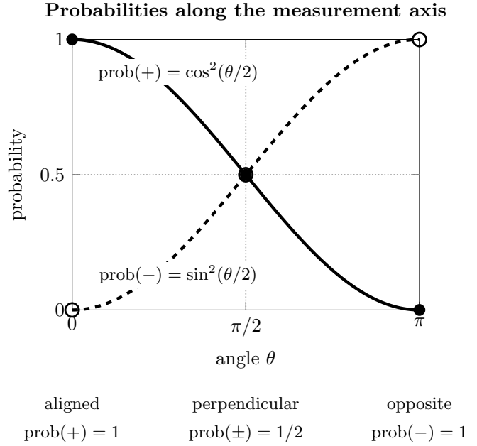
Figure 3: Spin prepared along \mathbf{u}' and measured along \mathbf{u} . Only the angle \theta between the axes enters the probabilities. The solid curve gives the +1/2 outcome; the dashed curve gives the -1/2 outcome. Aligned axes give certainty, perpendicular axes give equal probabilities, and opposite axes reverse the certain outcome. The two curves sum to one at every angle.
