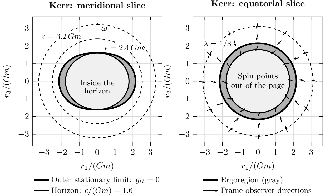
Figure 5: Kerr coordinate slices with spin along +r_3 and Gm\|\omega\| = 1/4 , so \ell^2\|\omega\| = 0.8Gm and the horizon is \epsilon = 1.6Gm . Left: the r_2 = 0 slice, with dashed black contours of the ellipsoidal radius \epsilon . Right: the r_3 = 0 slice, with a dashed constant- \lambda contour and equal-length arrows showing the direction of d\mathbf{r}/dt = -\lambda\mathbf{u}/(1+\lambda) . Solid black curves mark the horizon and outer stationary limit, with the exterior ergoregion shaded gray. Pale gray marks the horizon's interior. The arrows describe the chosen frame observers, not general free fall; the coordinate shapes are not an isometric embedding.
