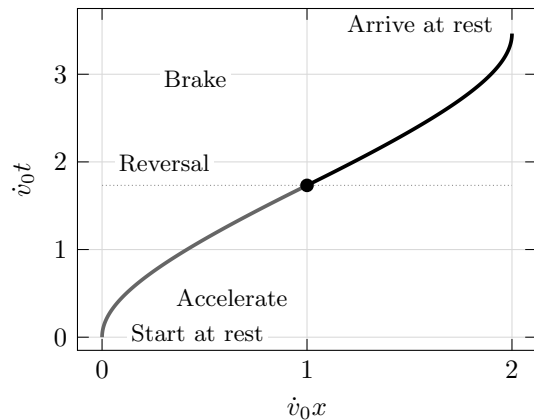
One trip; thrust reverses halfway
