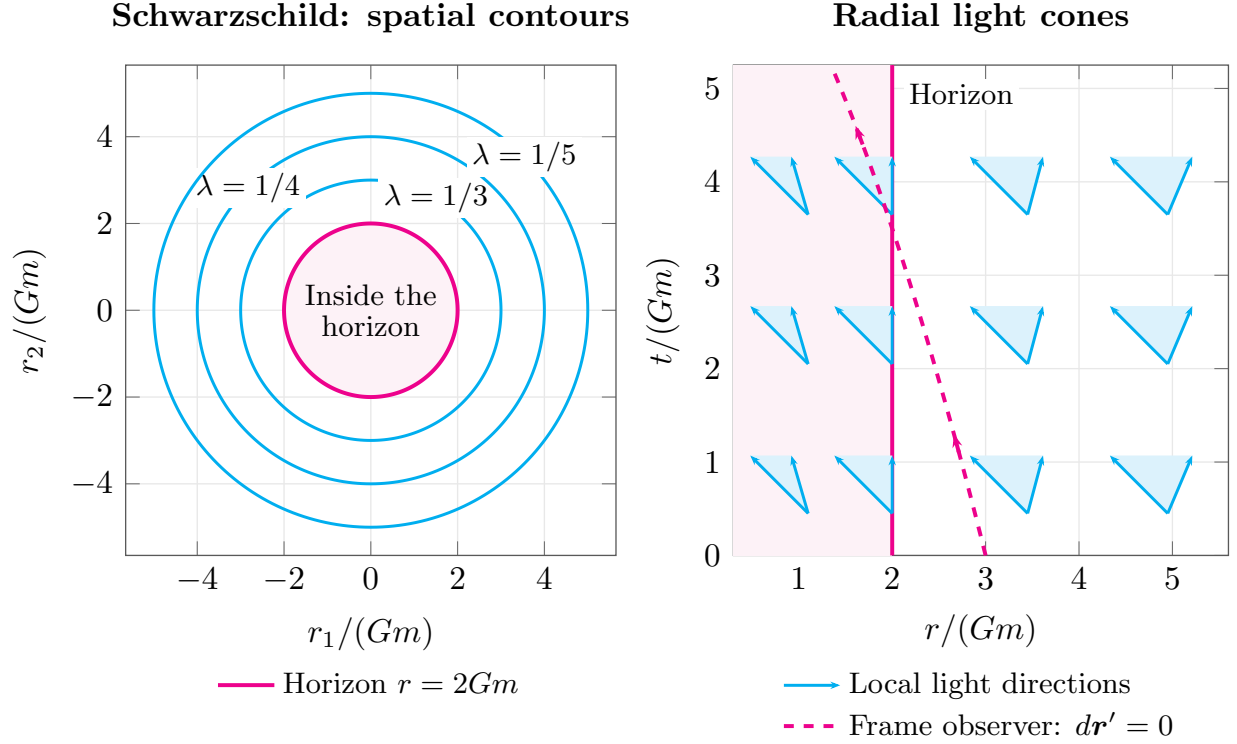
Figure 2: Schwarzschild in the coordinates of (19.28), with lengths and times in units of Gm . Left: constant- \lambda circles in the r_3 = 0 plane; the solid magenta circle is the horizon, with its interior shaded pale magenta. Right: future radial light cones, drawn as local tangent directions, with time increasing upward. The dashed magenta curve follows the chosen frame observer, dr/dt = -Gm/(r + Gm) , starting at r = 3Gm when t = 0 ; it is not a free-fall trajectory. The spatial panel shows coordinate contours, not proper distances or an isometric embedding.
