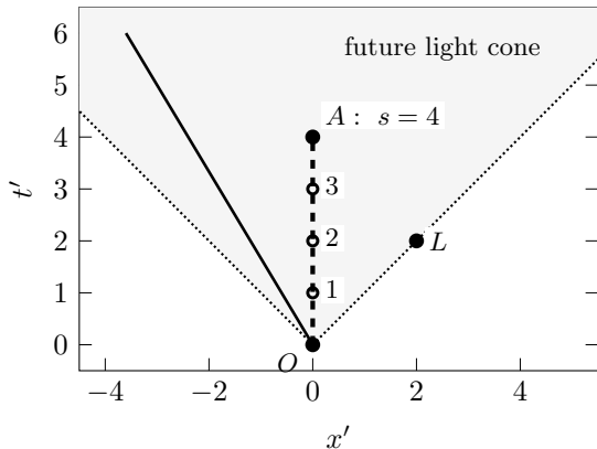
Moving clock's rest frame
