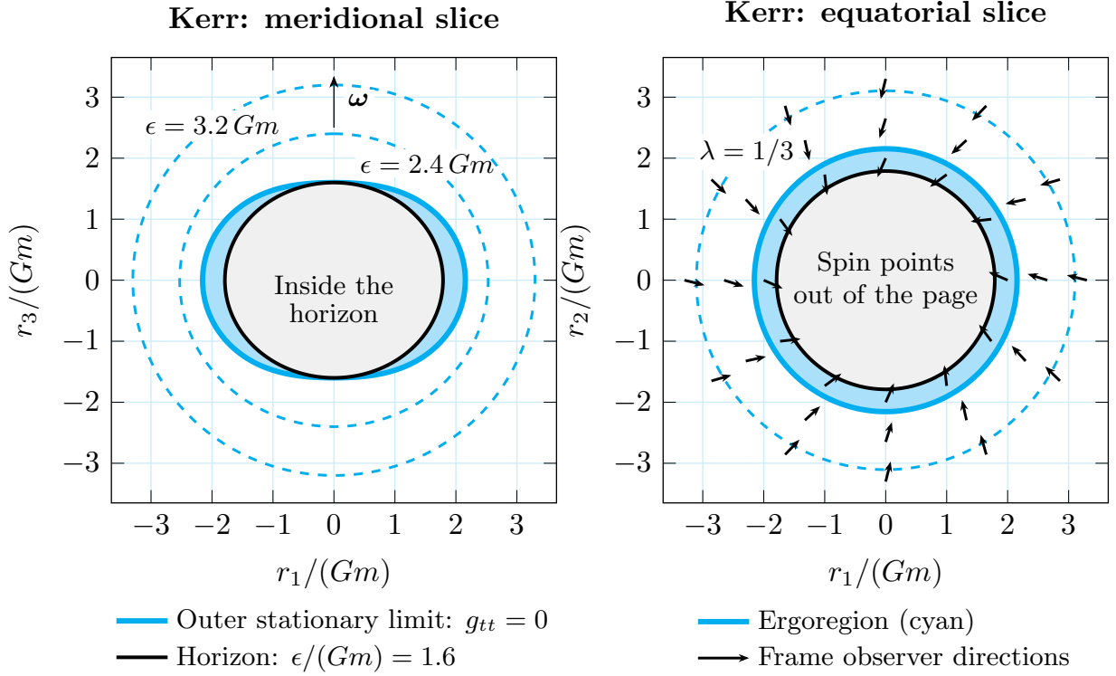
Figure 5: Kerr coordinate slices with spin along +r_3 and Gm\|\omega\| = 1/4 , so \ell^2\|\omega\| = 0.8Gm and the horizon is \epsilon = 1.6Gm . Left: the r_2 = 0 slice, with dashed cyan contours of the ellipsoidal radius \epsilon . Right: the r_3 = 0 slice, with a dashed constant- \lambda contour and equal-length arrows showing the direction of d\mathbf{r}/dt = -\lambda\mathbf{u}/(1+\lambda) . Solid black marks the horizon; solid cyan marks the outer stationary limit, with the exterior ergoregion shaded pale cyan. Pale gray marks the horizon's interior. The arrows describe the chosen frame observers, not general free fall; the coordinate shapes are not an isometric embedding.
