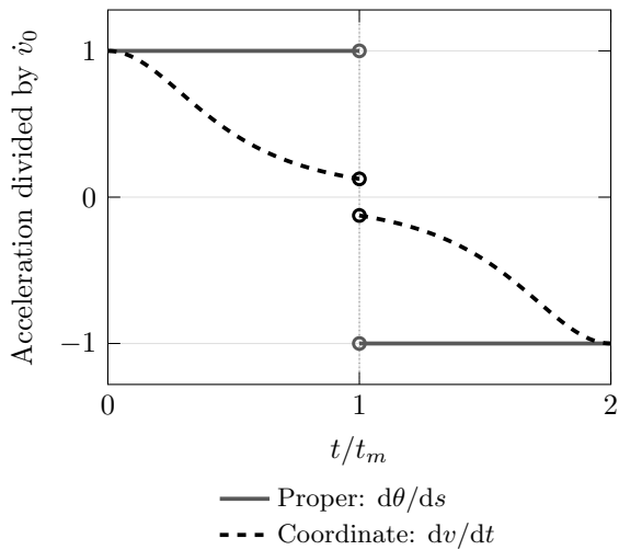
Proper and coordinate acceleration
