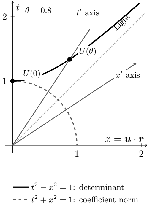
Figure 1: Boost geometry in the t, x plane, with x = \mathbf{u} \cdot \mathbf{r} . The gray primed axes have rapidity \theta = 0.8 . The vector U = L^{-2} is the primed frame's unit time direction, expressed in the original coordinates; its components lie on the solid black unit-determinant hyperbola. The boost takes this vector to rest while preserving the light directions. The dashed unit-norm circle is not preserved. Right: \det U = 1 for every rapidity, whereas \|U\|^2 = \cosh(2\theta) changes.
