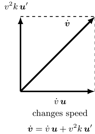
Figure 3: The Frenet frame follows the spatial path. At the marked point, the tangent \mathbf{u} and principal normal \mathbf{u}' lie in the osculating plane; \mathbf{u}'' points out of the page. The dashed osculating circle has radius 1/k . Smaller arrows show how the tangent and normal change along the path. Right: tangential acceleration changes speed, while normal acceleration changes direction. The example is planar, so \tau = 0 ; primes label frame vectors, not derivatives.
