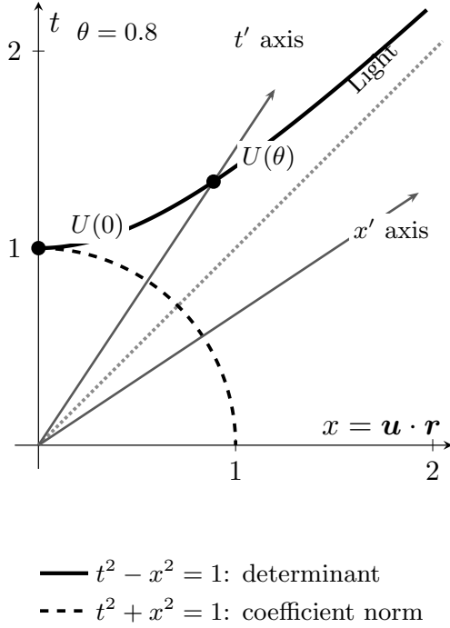
Figure 1: Boost geometry in the t, x plane, with x = \mathbf{u} \cdot \mathbf{r} \in \mathbb{R} . The gray primed axes have rapidity \theta = 0.8 . The vector U = L^{-2} is the primed frame's unit time direction, expressed in the original coordinates; its components lie on the black unit-determinant hyperbola. The boost takes this vector to rest while preserving the light directions. The dashed unit-norm circle is not preserved. Right: \det U = 1 for every rapidity, whereas \|U\|^2 = \cosh(2\theta) changes.
