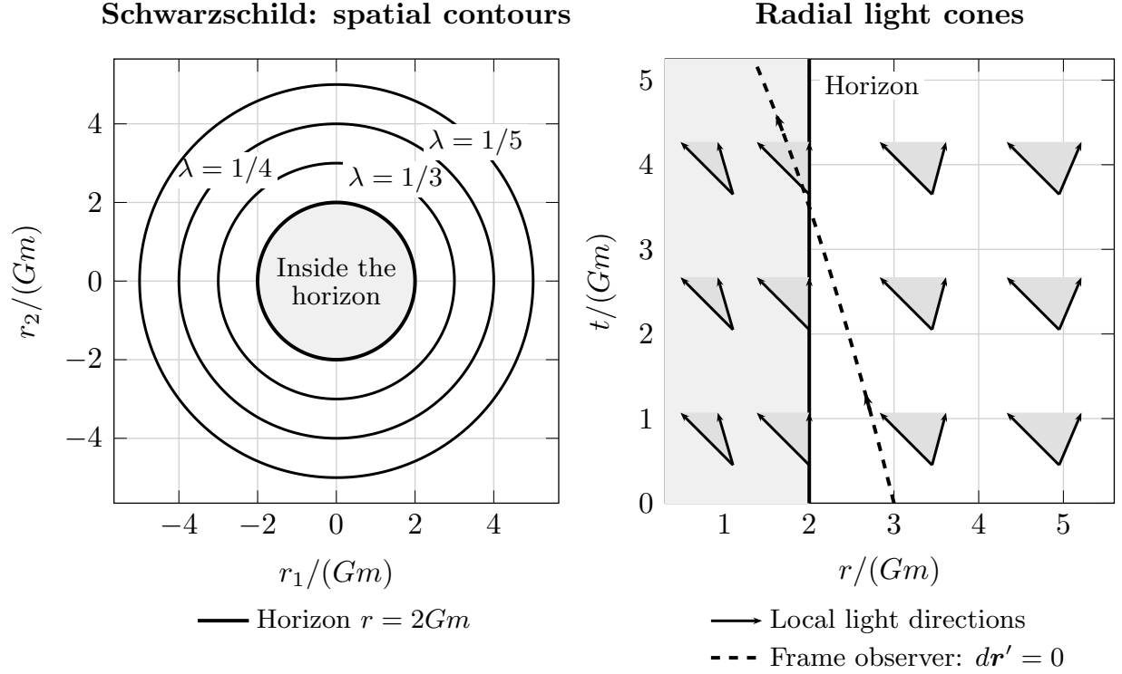
Figure 5: Schwarzschild in the coordinates of (19.28), with lengths and times in units of Gm . Left: constant- \lambda circles in the r_3 = 0 plane; the solid black circle is the horizon, with its interior shaded pale gray. Right: future radial light cones, drawn as local tangent directions, with time increasing upward. The dashed black curve follows the chosen frame observer, dr/dt = -Gm/(r + Gm) , starting at r = 3Gm when t = 0 ; it is not a free-fall trajectory. The spatial panel shows coordinate contours, not proper distances or an isometric embedding.
