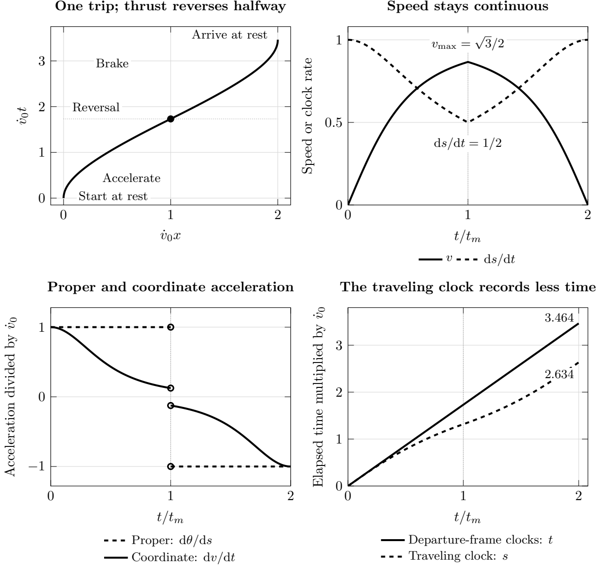
Figure 2: Midpoint braking in flat spacetime, with x = \mathbf{u} \cdot \mathbf{r} \in \mathbb{R} and \dot{v}_0 \ell = 2 . Dotted guides mark the reversal at t = t_m . The trajectory and speed remain continuous while the signed acceleration changes abruptly; open circles show its one-sided values. The proper-acceleration magnitude stays fixed, whereas |\dot{v}| = \dot{v}_0/\gamma^3 varies. The reduced clock rate accumulates to a shorter onboard elapsed time. All plotted axes use the natural units of the main text.
