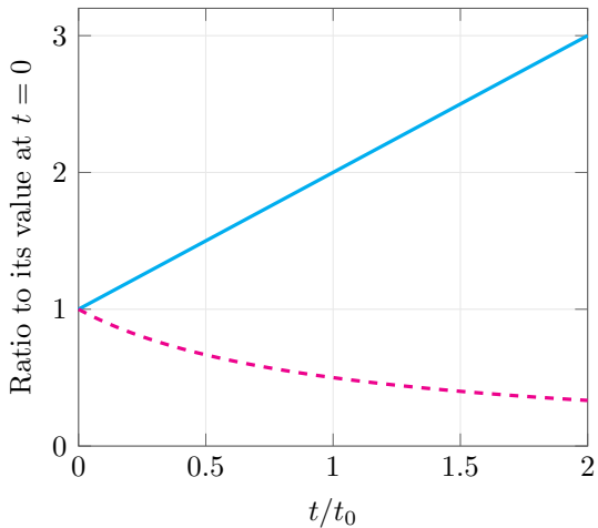
Separation and momentum
