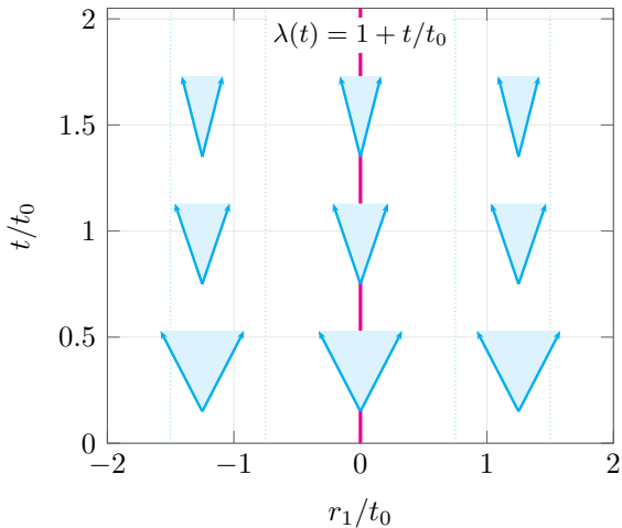
Expansion: local light cones
