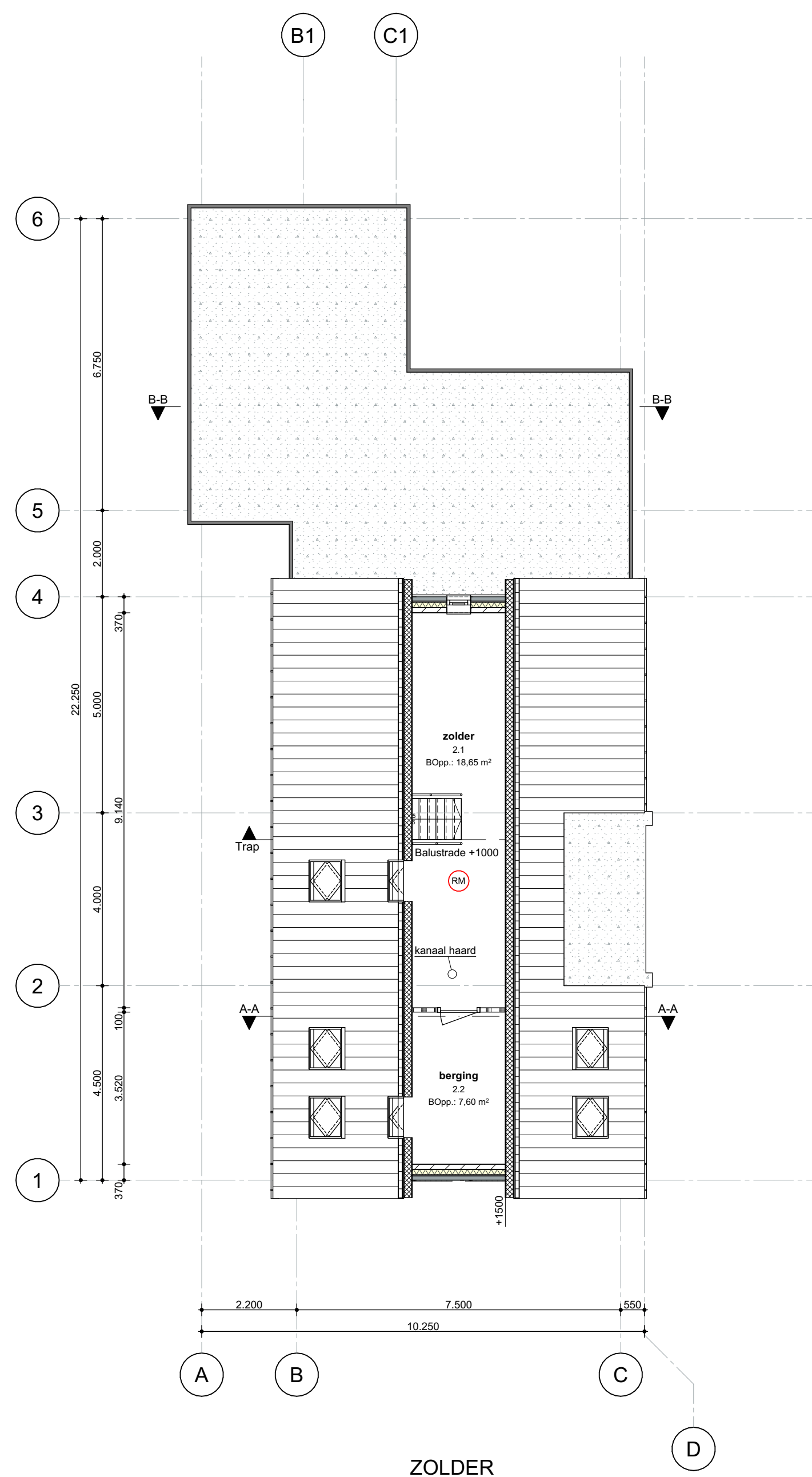
ZOLDER
