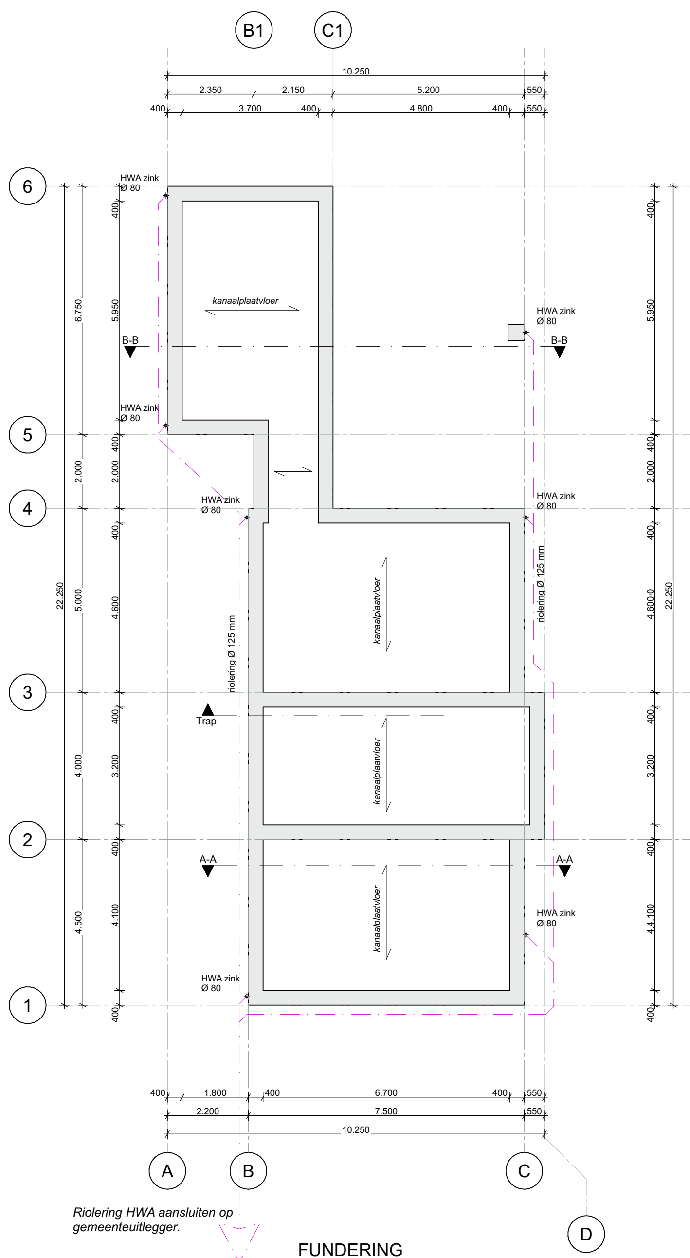
FUNDERING
