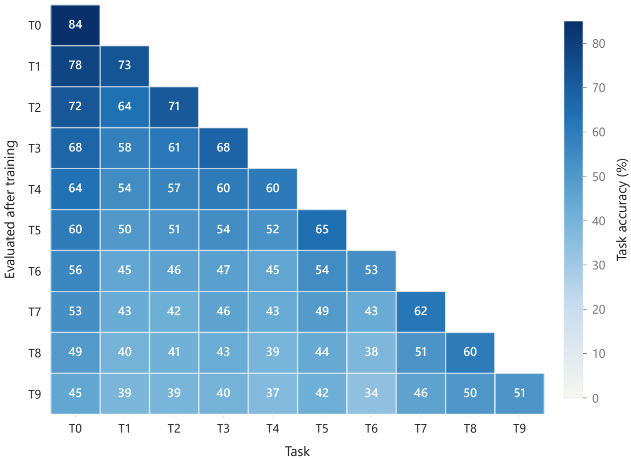
iCaRL — task evolution (steady diagonal erosion)
