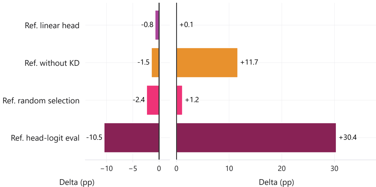
(a) Delta average accuracy (pp)
