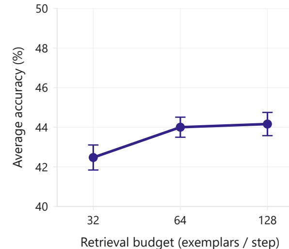
(c) Retrieval budget — Accuracy
