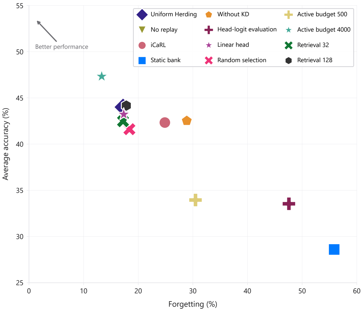
Accuracy vs. Forgetting Trade-off
