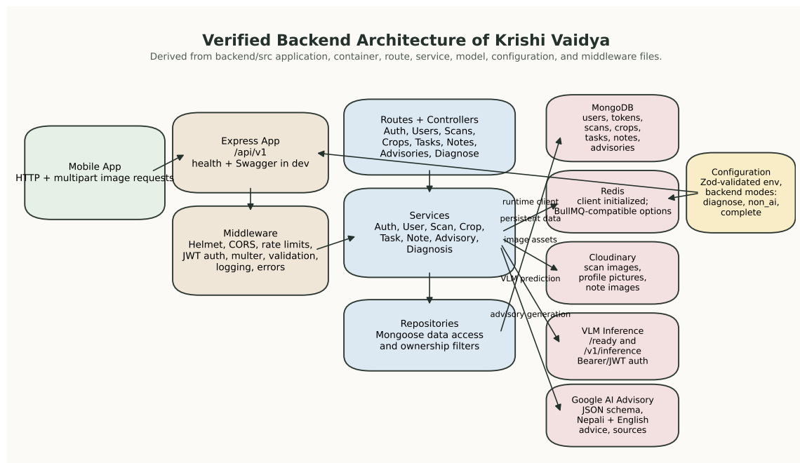
Figure 1: Verified backend architecture of Krishi Vaidya
