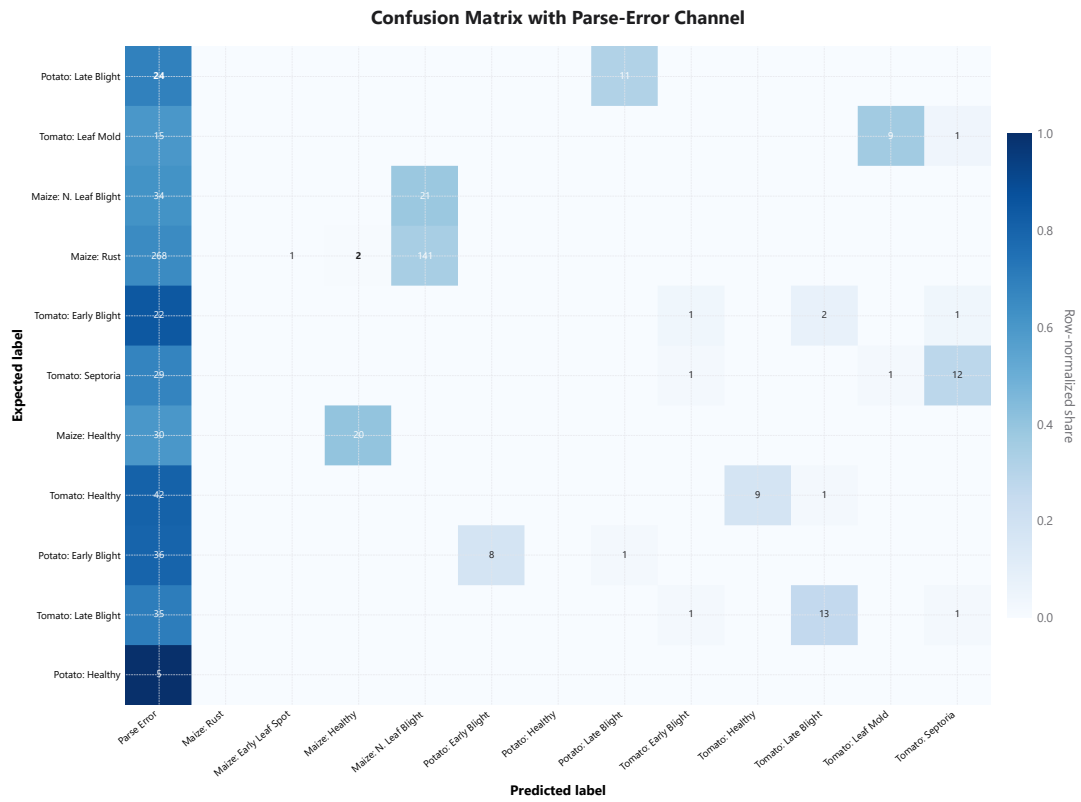
Figure 13: Confusion matrix for VLM prediction results
