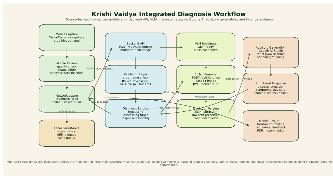
Figure 3: Integrated Krishi Vaidya diagnosis workflow across mobile app, backend API, VLM inference gateway, advisory generation, and local persistence.
