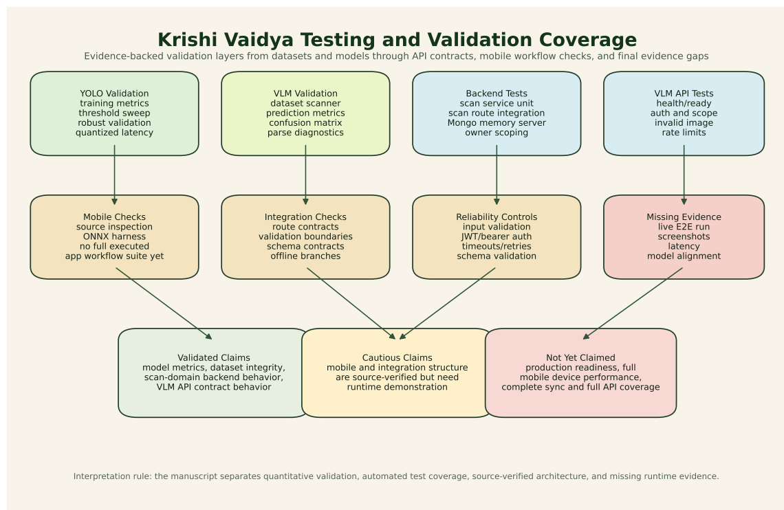
Figure 4: Testing and validation coverage across model, backend, mobile, API, and integration layers.
