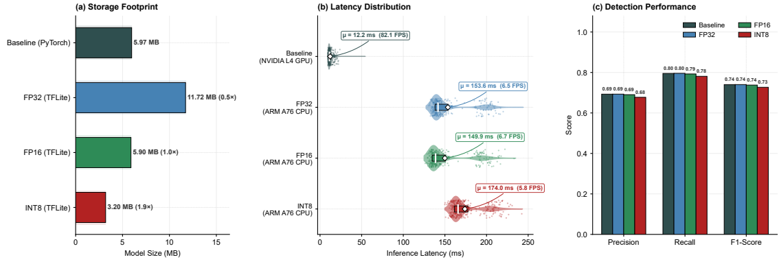
Figure 7: Deployment comparison across baseline and quantized YOLO variants
