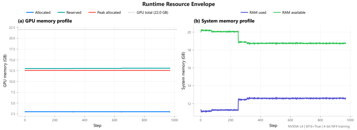
Figure 10: Runtime and memory behavior of the VLM training run
