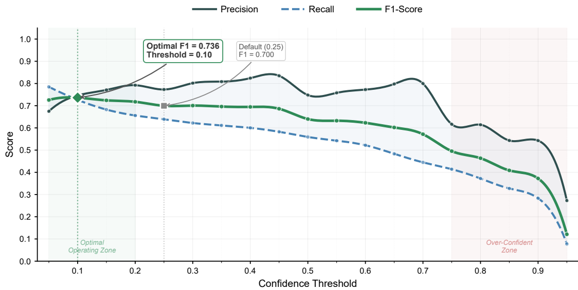
Figure 6: Confidence-threshold sensitivity of the YOLO detector
