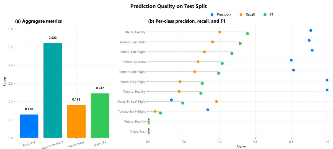
Figure 12: Prediction performance of the VLM on the test split
