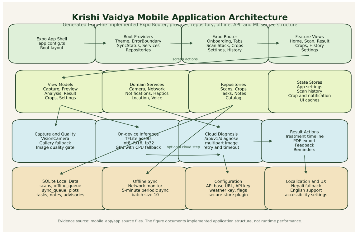
Figure 2: Mobile application architecture generated from the implemented Expo, provider, repository, of- fline, API, and ML source structure.
