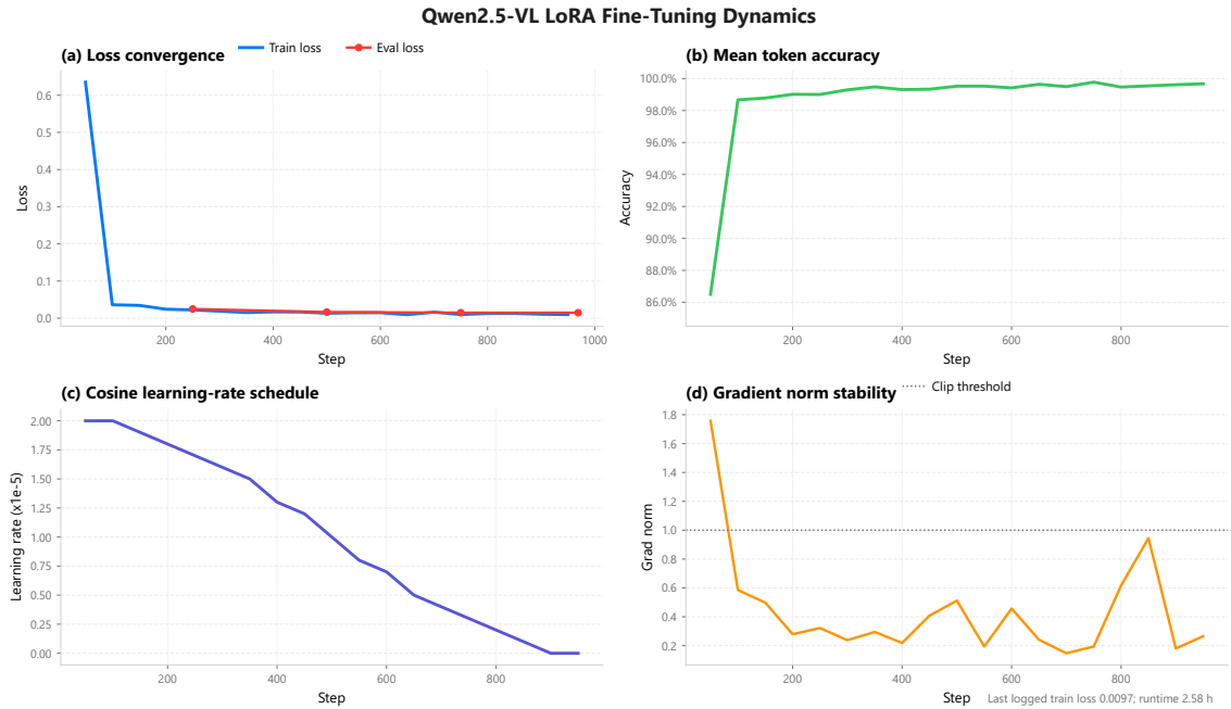
Figure 9: Training dynamics of the Qwen2.5-VL LoRA fine-tuning run
