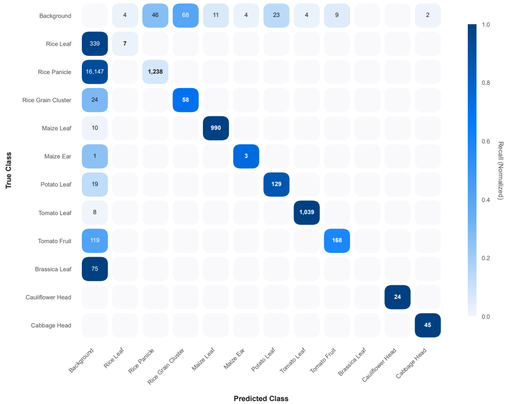
Figure 8: Confusion matrix of the YOLO detector
