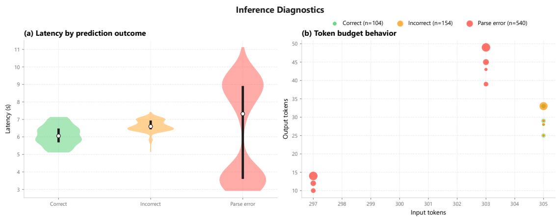
Figure 14: Inference diagnostics for VLM predictions
