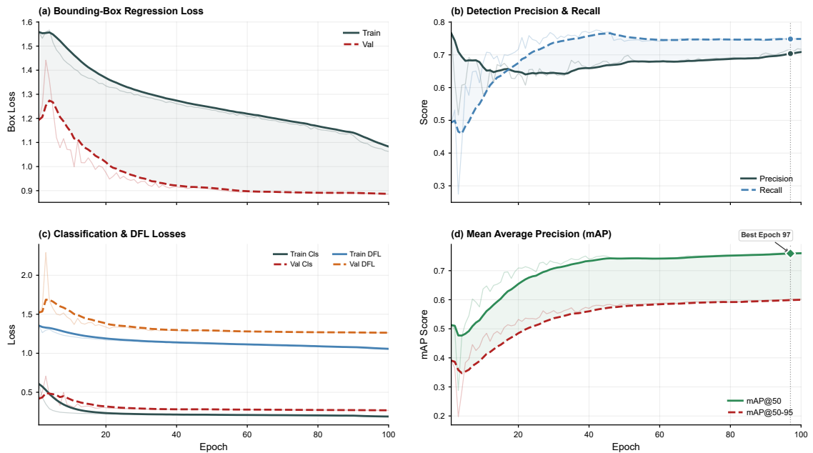
Figure 5: Training dynamics of the Krishi Vaidya YOLO detector
