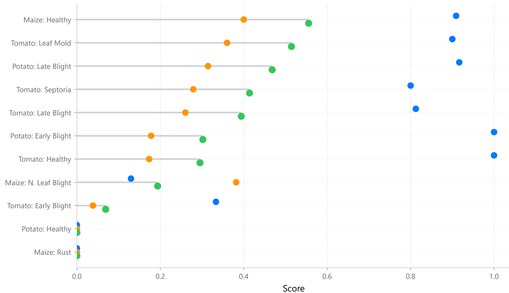
(b) Per-class precision, recall, and F1
