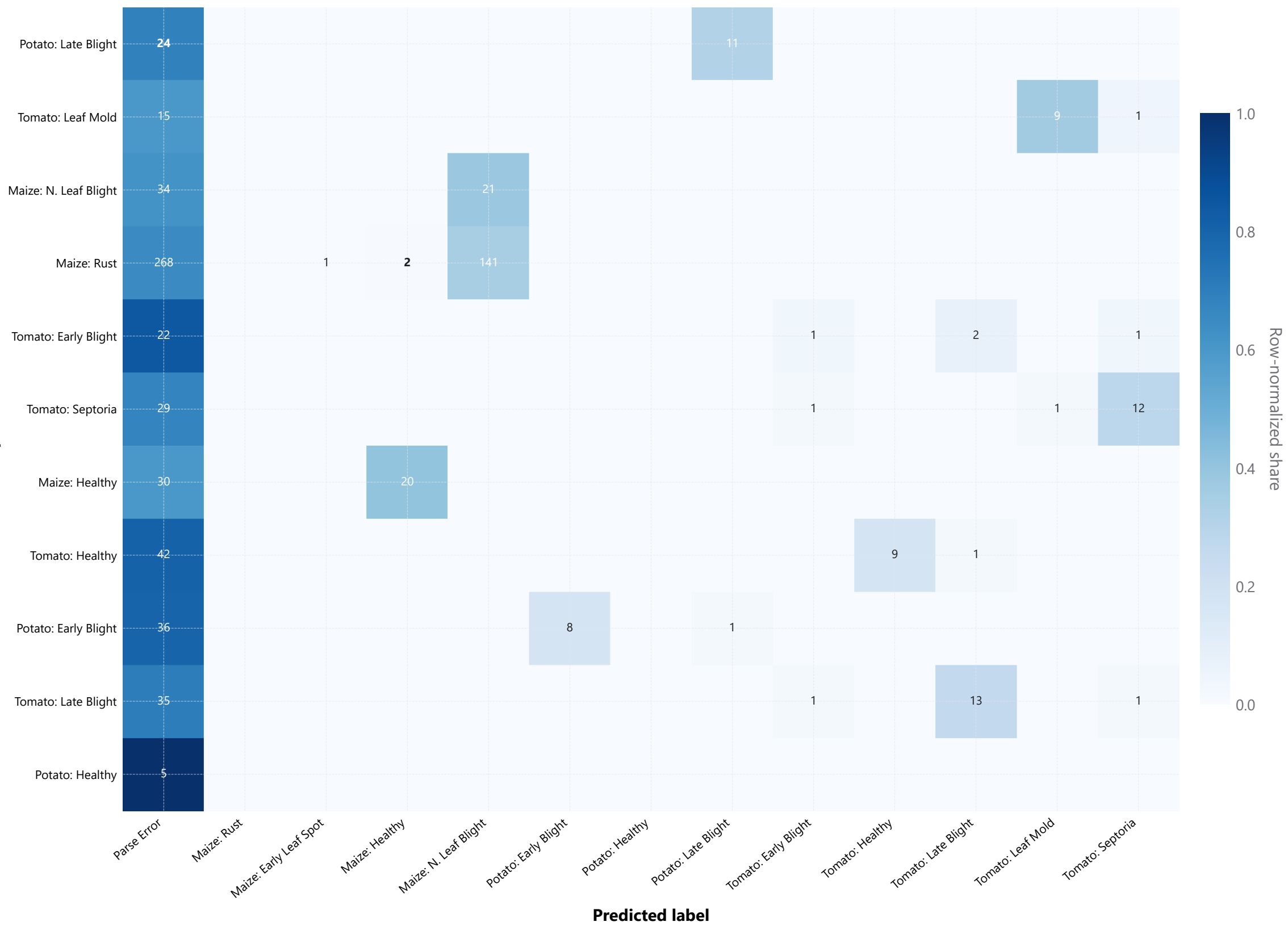
Confusion Matrix with Parse-Error Channel
