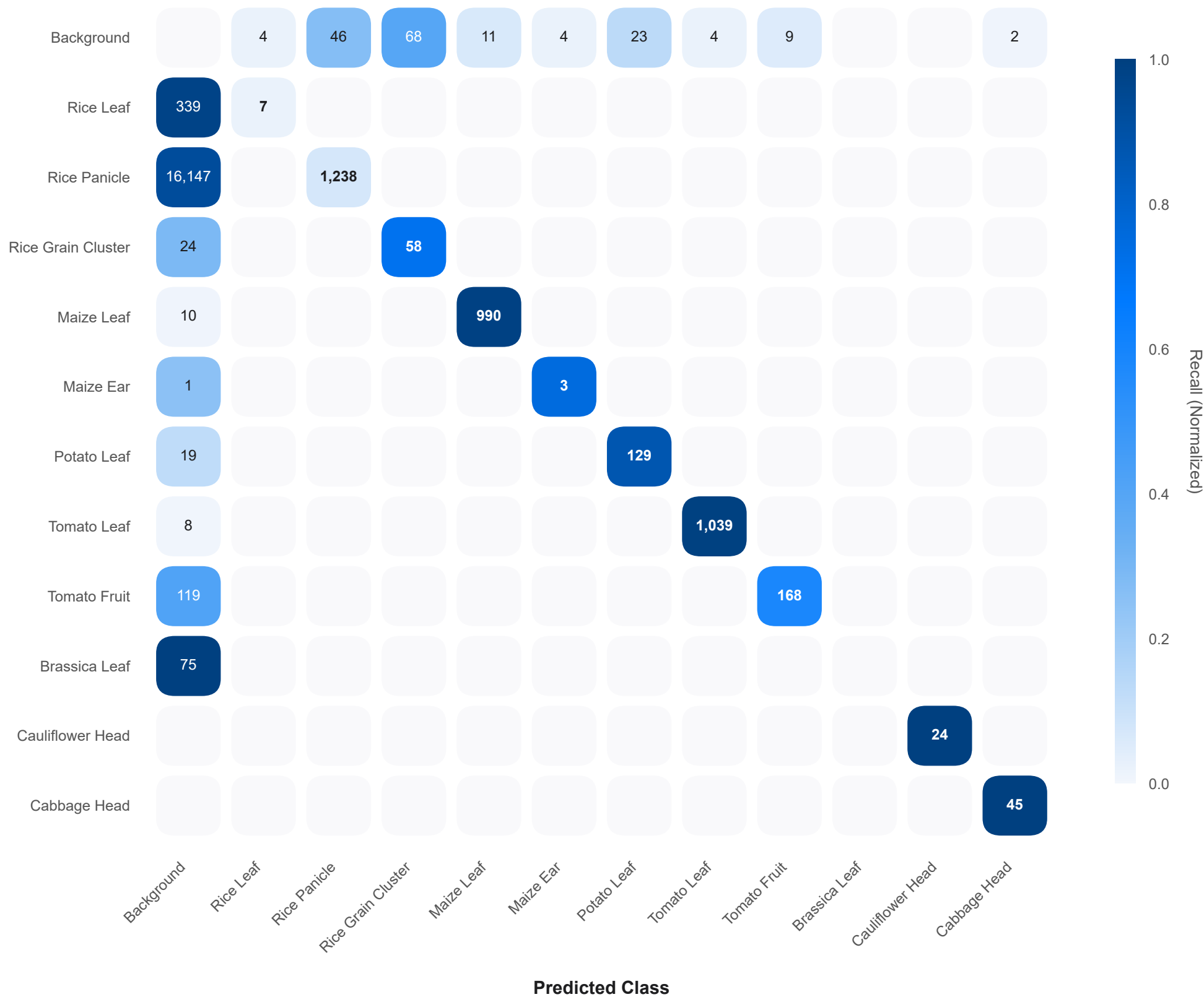
Figure 4: Baseline Model Confusion Matrix
