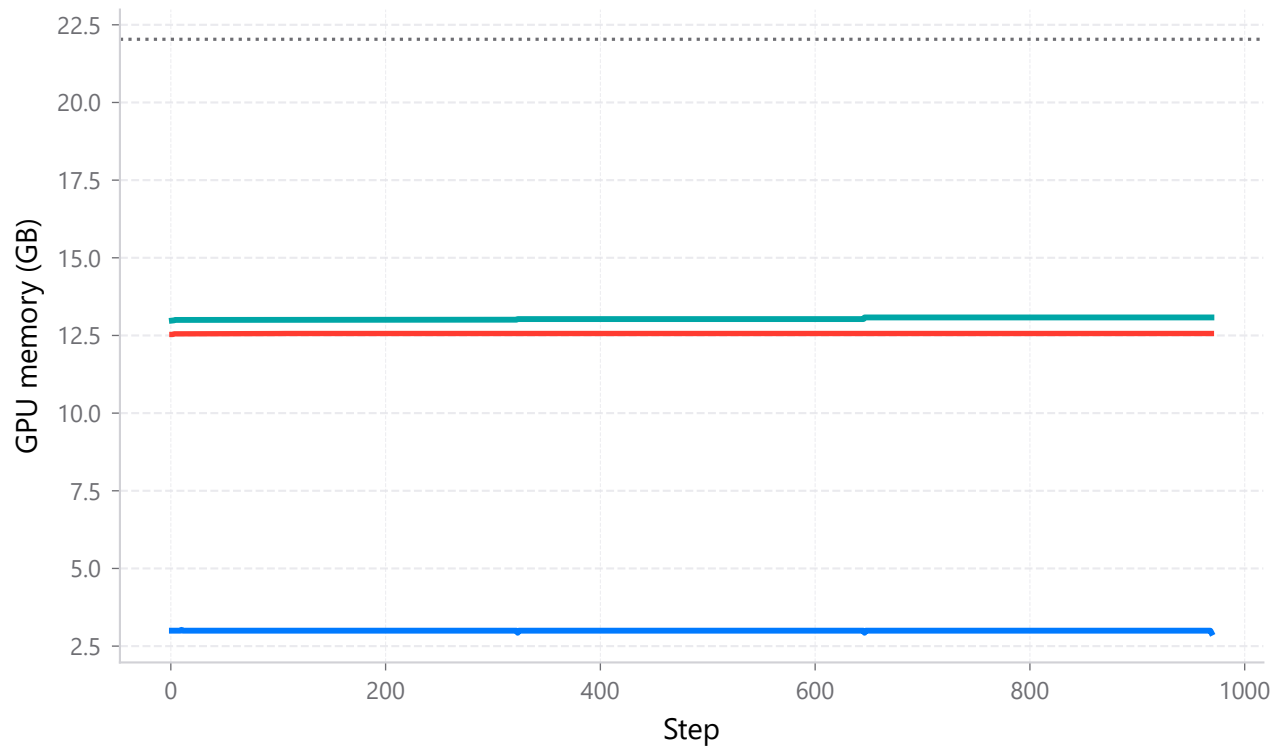
(a) GPU memory profile
